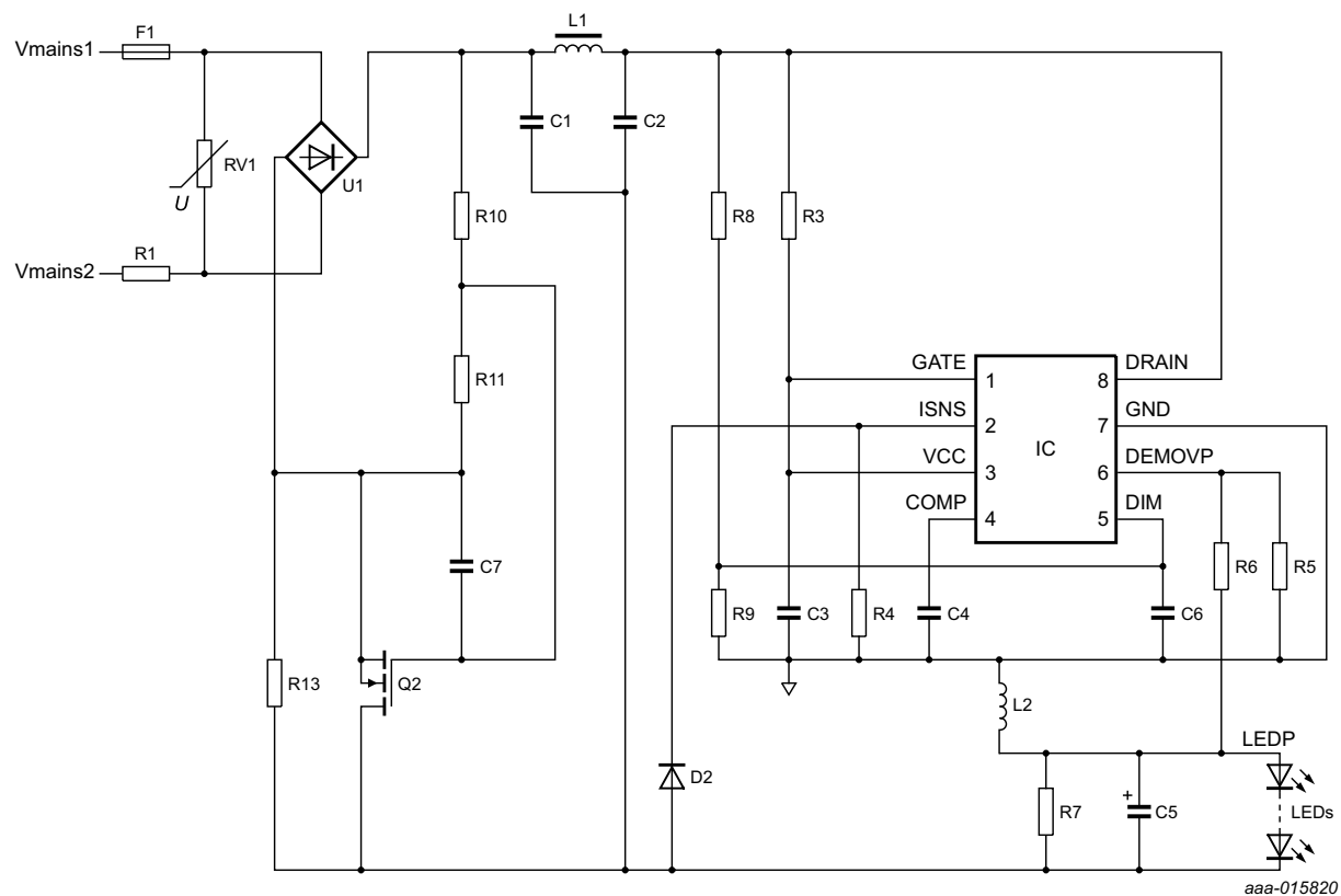
Fig 7. SSL5236BTE typical application diagram
