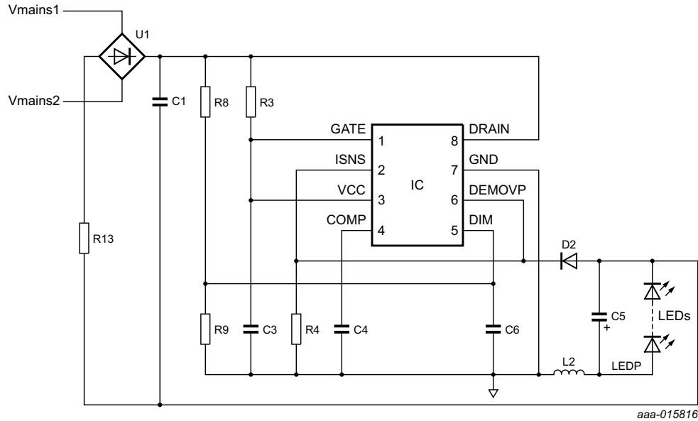
Fig 3. SSL5236BTE basic application diagram
