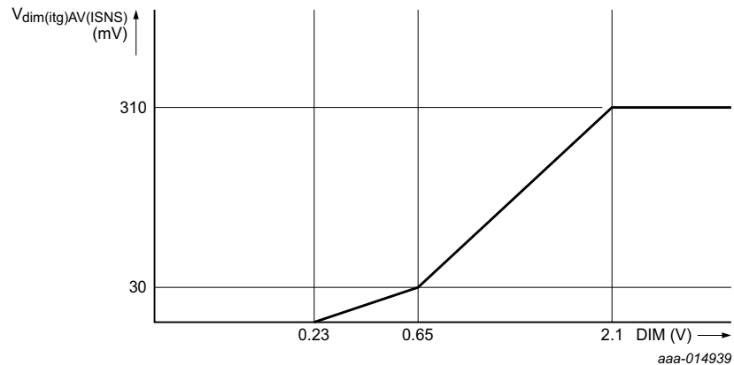
Fig 4. Dimming control transfer function
