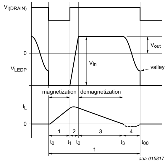
Fig 5. buck waveforms and valley detection
