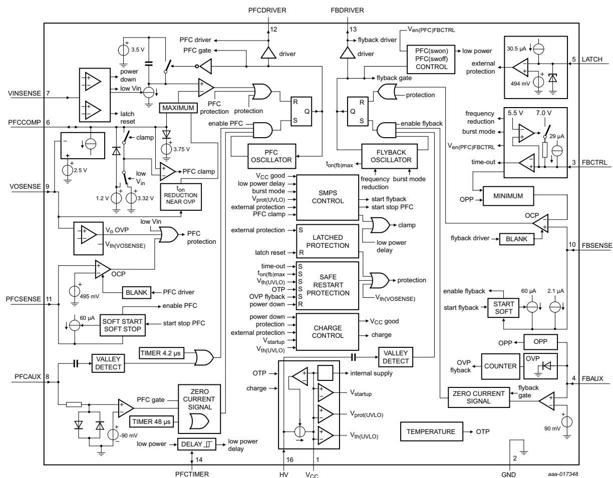
Fig 1. SSL8516BT block diagram
