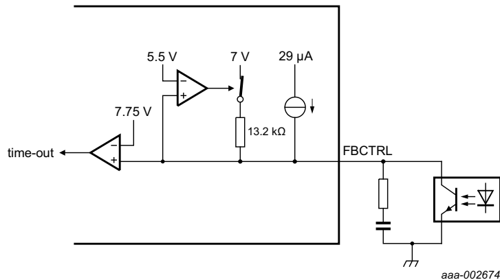
Fig 11. Time-out protection circuit
