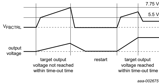
Fig 12. SSL8516BT time-out protection (signals) and safe restart
