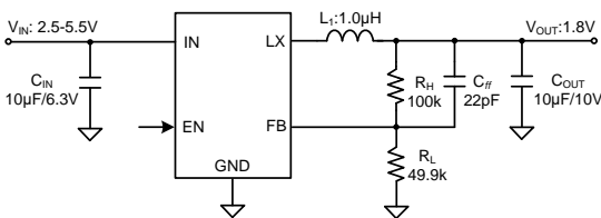
Figure1. Schematic Diagram
