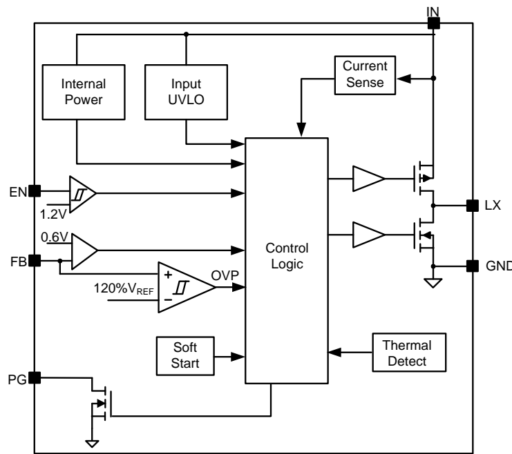
Figure3. Block Diagram
