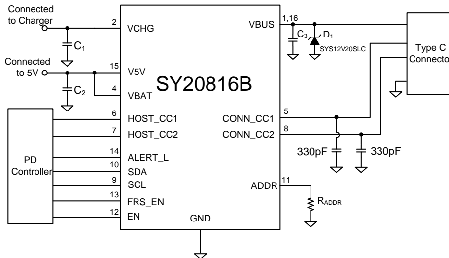
Fig.1 Schematic diagram
