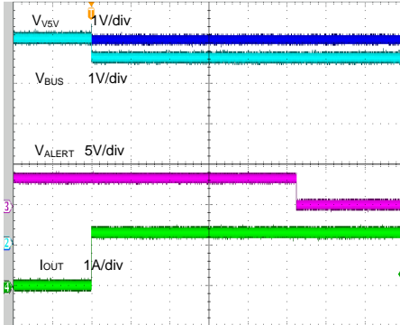
V5V Channel Over Current Response ( V_{V5V}=5V , V5V Source mode, 5V\_ILIM=00 , OC\_DELAY=10 , 3.5Ω switch on)
