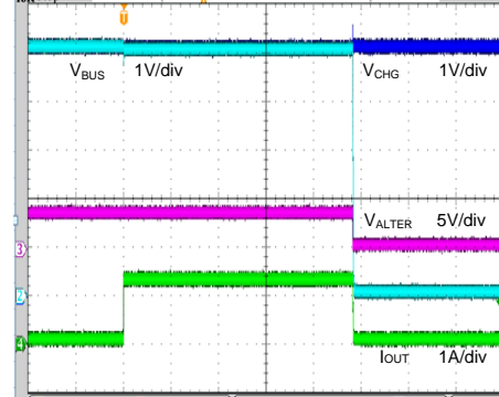
CHG Channel Over Current Response ( V_{CHG}=5V , CHG\_ILIM=00 , DSG\_Time=00 , OC\_DELAY=10 , CHG Source mode, C_{CHG}=C_{BUS}=10\mu F , 3.5Ω switch on)
