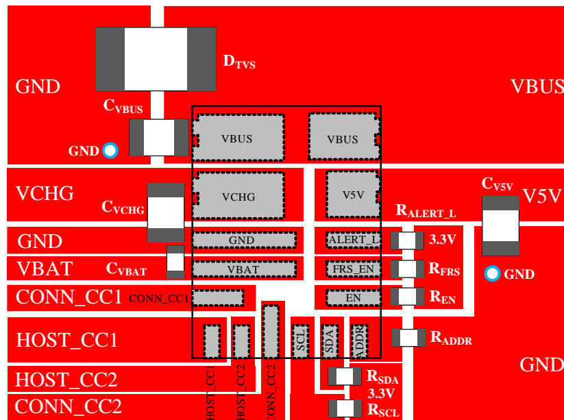
Fig.9 PCB Layout Suggestion
