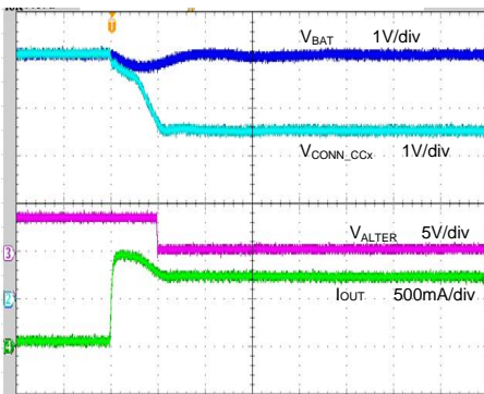
VCONN Channel Over Current Response ( V_{BAT}=5V , C_{BAT}=1\mu F , Load=5Ω ON)
