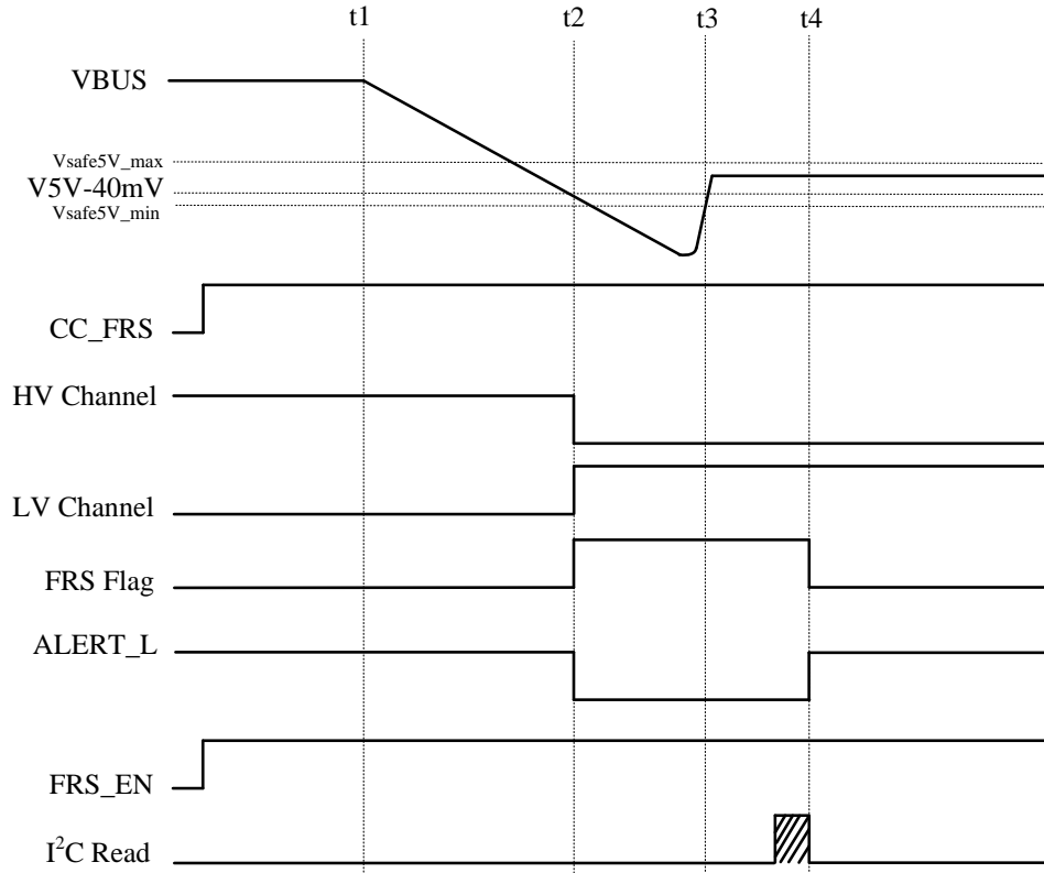
Figure 8. Timing Diagram on CC_FRS=1
