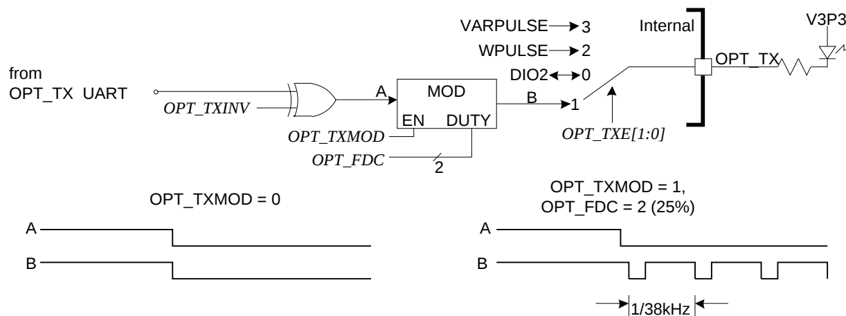
Figure 14: Optical Interface
