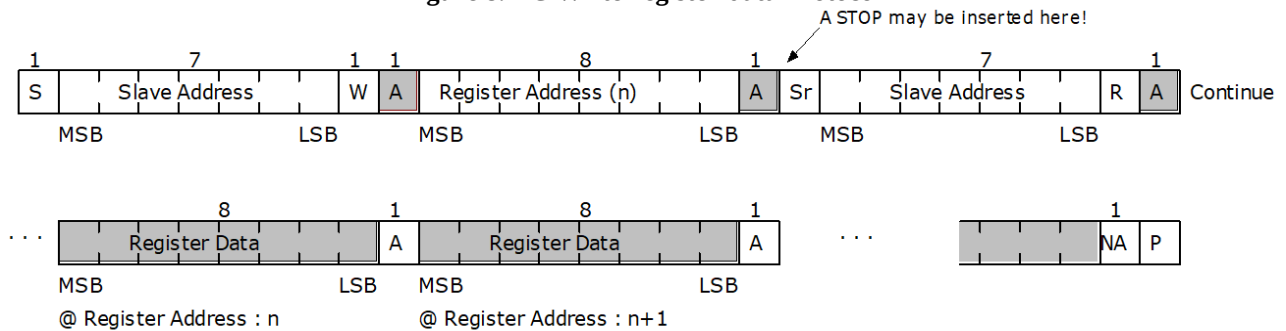
Figure 9. I 2 C Read-register-data Proctol
