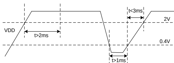
Figure 7. Power on Sequence
