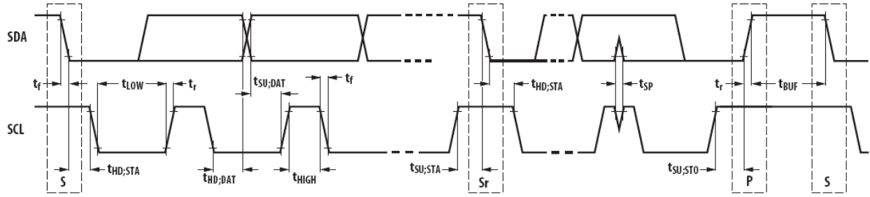
Figure 3. I²C Timing Diagram
