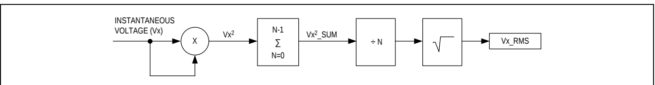
Figure 7. True RMS Value
