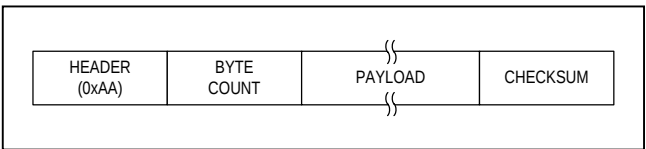
Figure 18. Master Packets
