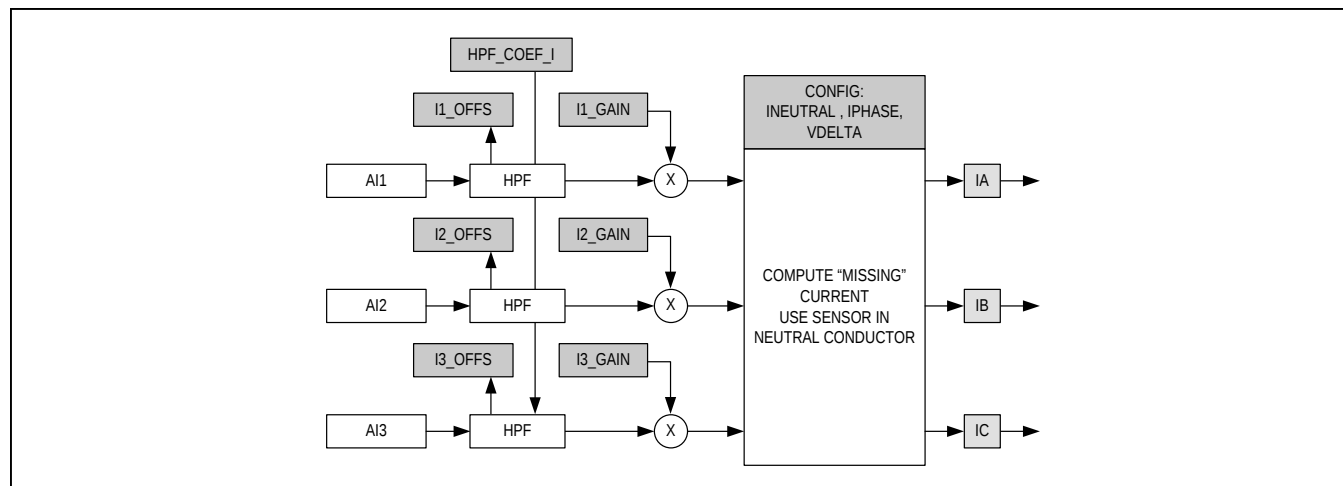
Figure 6. Computational Flowchart for IA, IB, and IC
