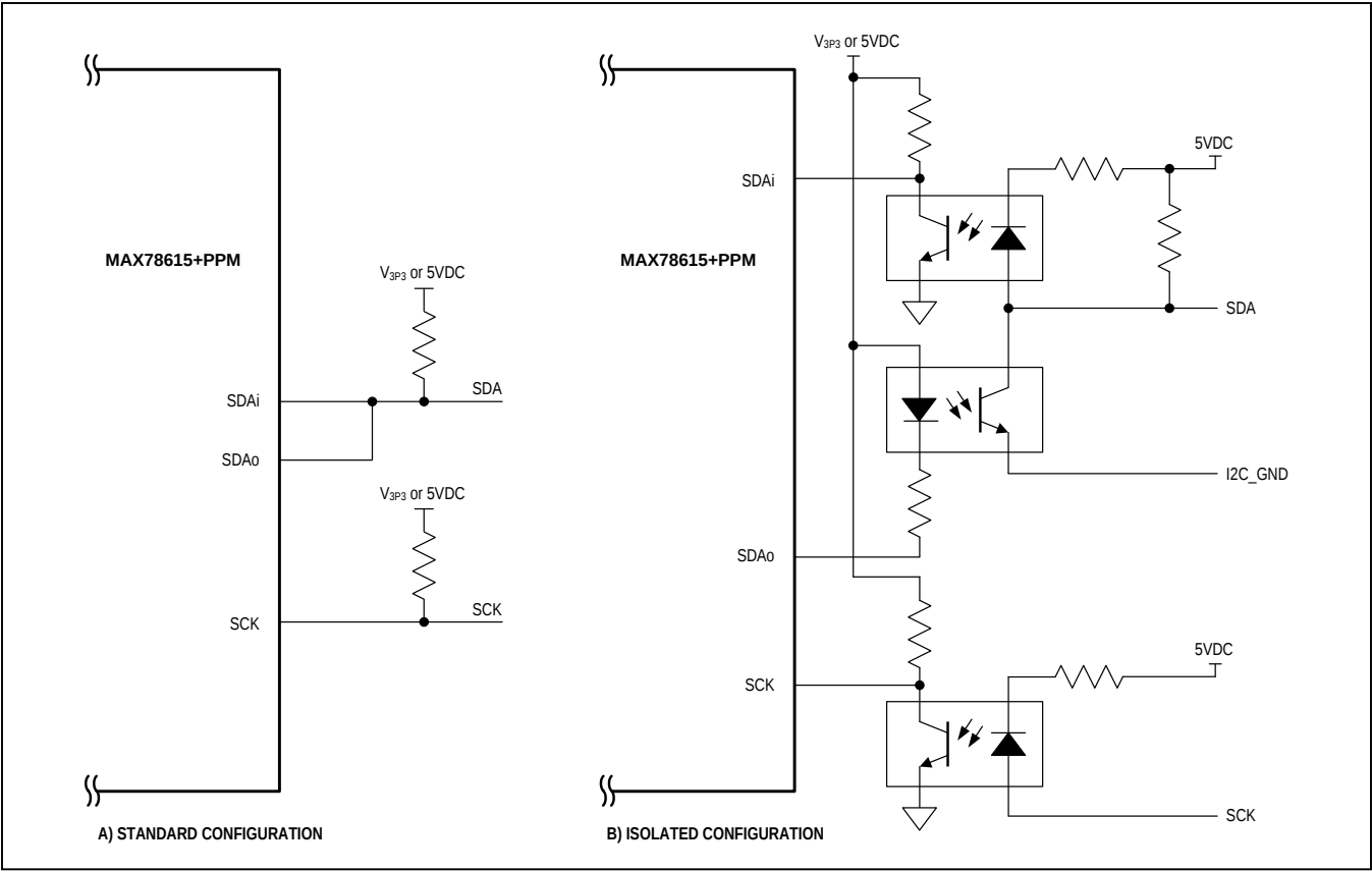
Figure 22. Configurations for I 2 C Interface
