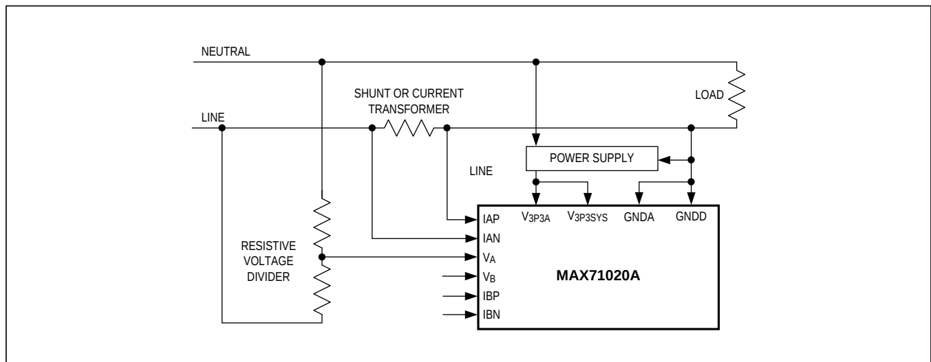
Figure 3. Typical Connection Diagram
