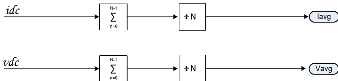
Figure 4-4: RMS Calculations
