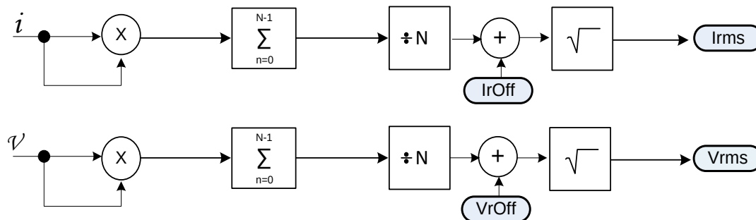
Figure 4-3: RMS Calculations
