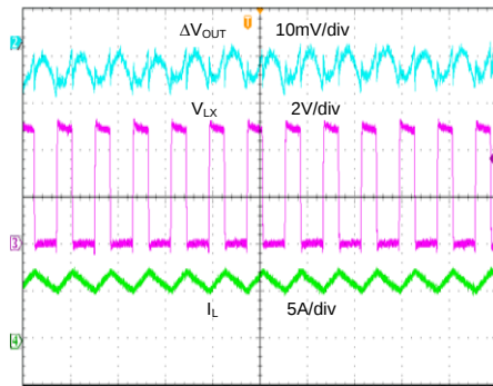
Output Ripple ( V_{IN}=5V , V_{OUT}=1.8V , I_{OUT}=6A )
