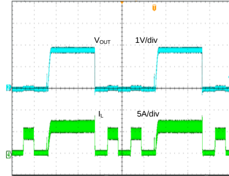
Short Circuit Protection ( V_{IN}=5V , V_{OUT}=1.8V , 6A to Short)
