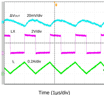
Output Ripple ( V_{IN} = 1.5\text{V} , V_{OUT} = 3.3\text{V} , I_{OUT} = 50\text{mA} )
