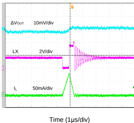
Output Ripple ( V_{IN} = 1.5\text{V} , V_{OUT} = 3.3\text{V} , I_{OUT} = 0\text{A} )
