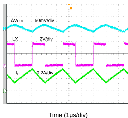
Output Ripple ( V_{IN} = 1.5\text{V} , V_{OUT} = 3.3\text{V} , I_{OUT} = 100\text{mA} )
