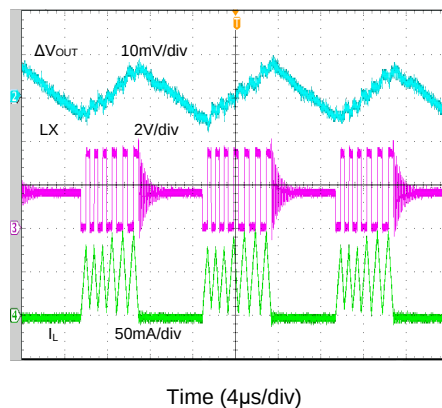
Output Ripple ( V_{IN} = 1.5\text{V} , V_{OUT} = 3.3\text{V} , I_{OUT} = 10\text{mA} )
