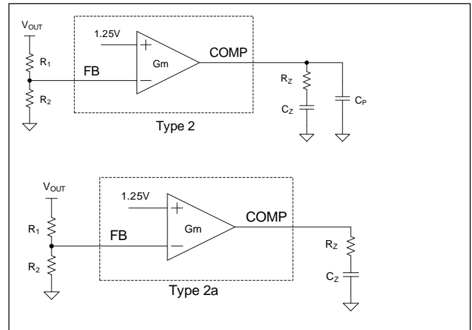
Figure 3. Compensation networks
