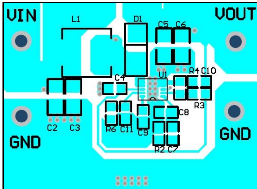
Figure 4. Recommended PCB Layout
