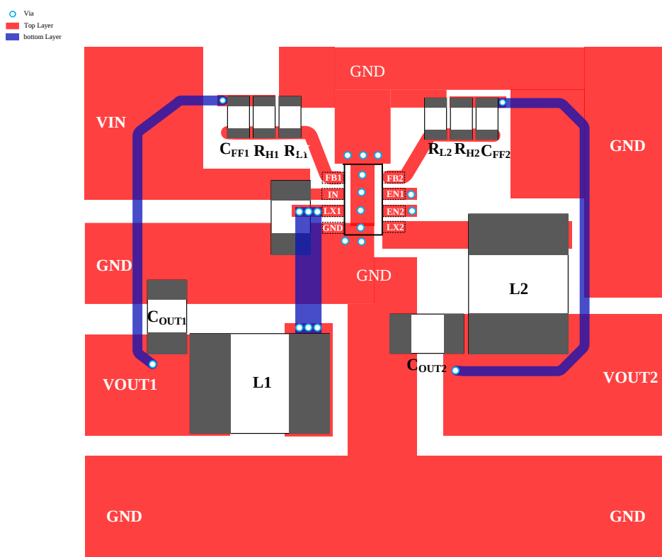
Figure3. PCB Layout Suggestion
