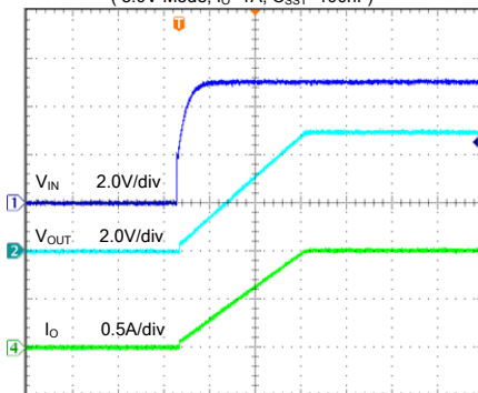
Programmable Soft-start Time (5.0V Mode, I_O=1A , C_{SST}=100nF )
