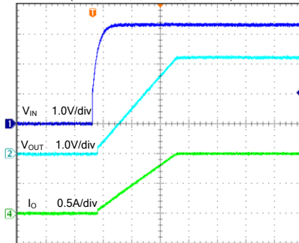
Programmable Soft-start Time (3.3V Mode, I_O=1A , C_{SST}=100nF )
