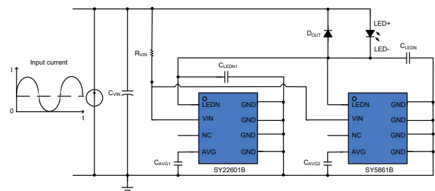
Fig3. Parallel circuit
