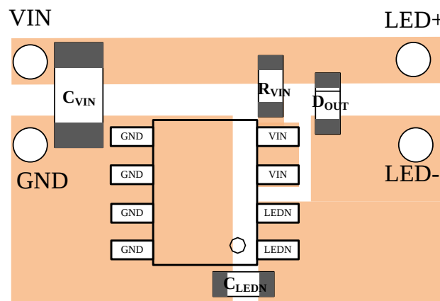
Figure 4. Recommend PCB Layout
