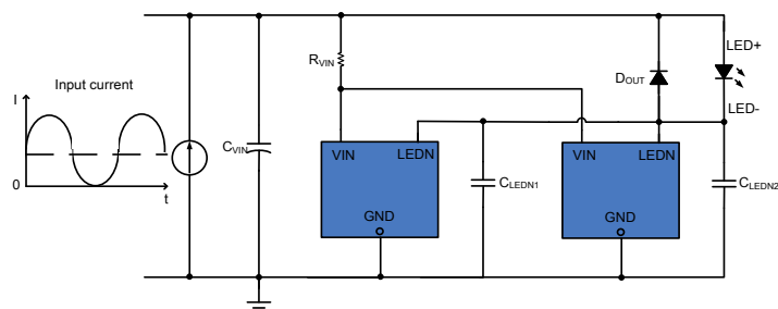
Figure 3. Parallel Circuit
