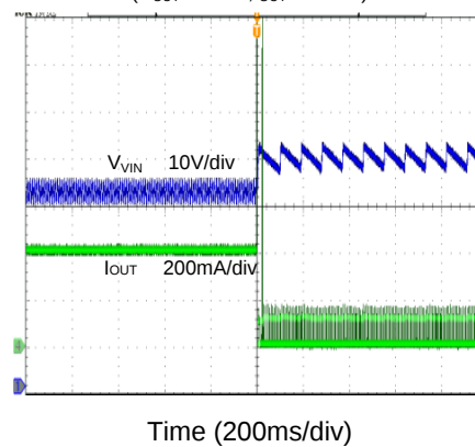
Short LED Protection ( C_{OUT}=660\mu F, I_{OUT}=500mA )
