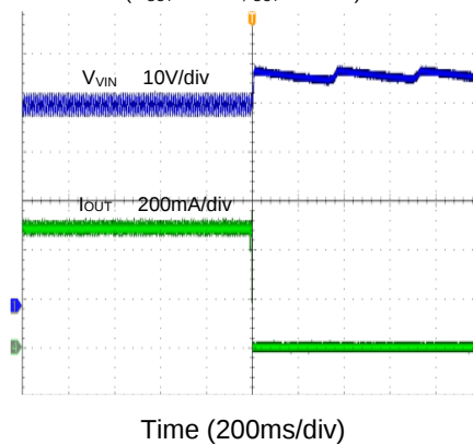
Open LED Protection ( C_{OUT}=660\mu F, I_{OUT}=500mA )
