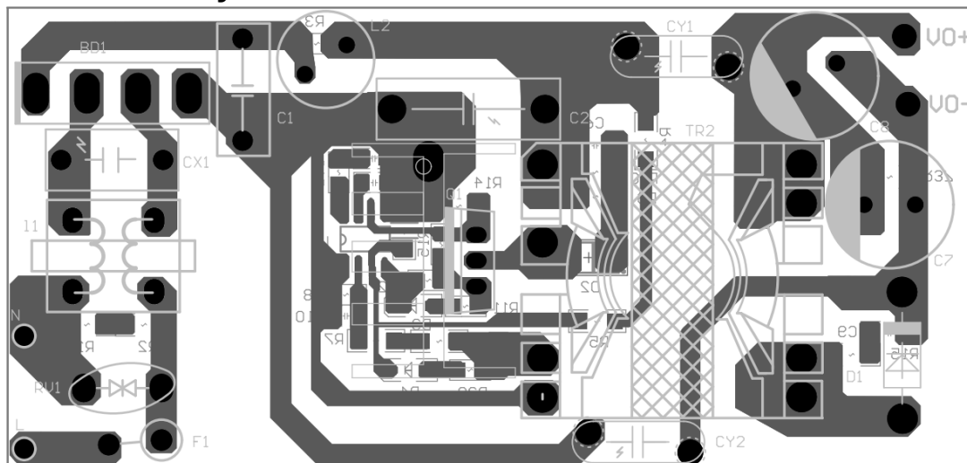
Figure 13. EVB Layout
