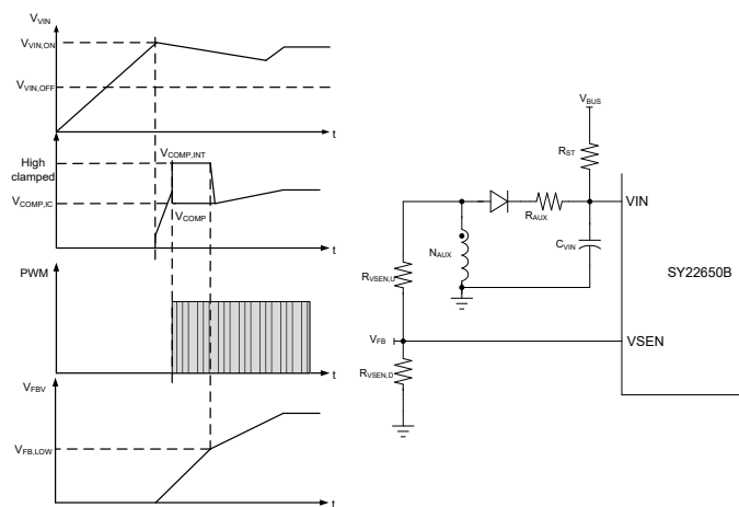
Figure 3. Startup
