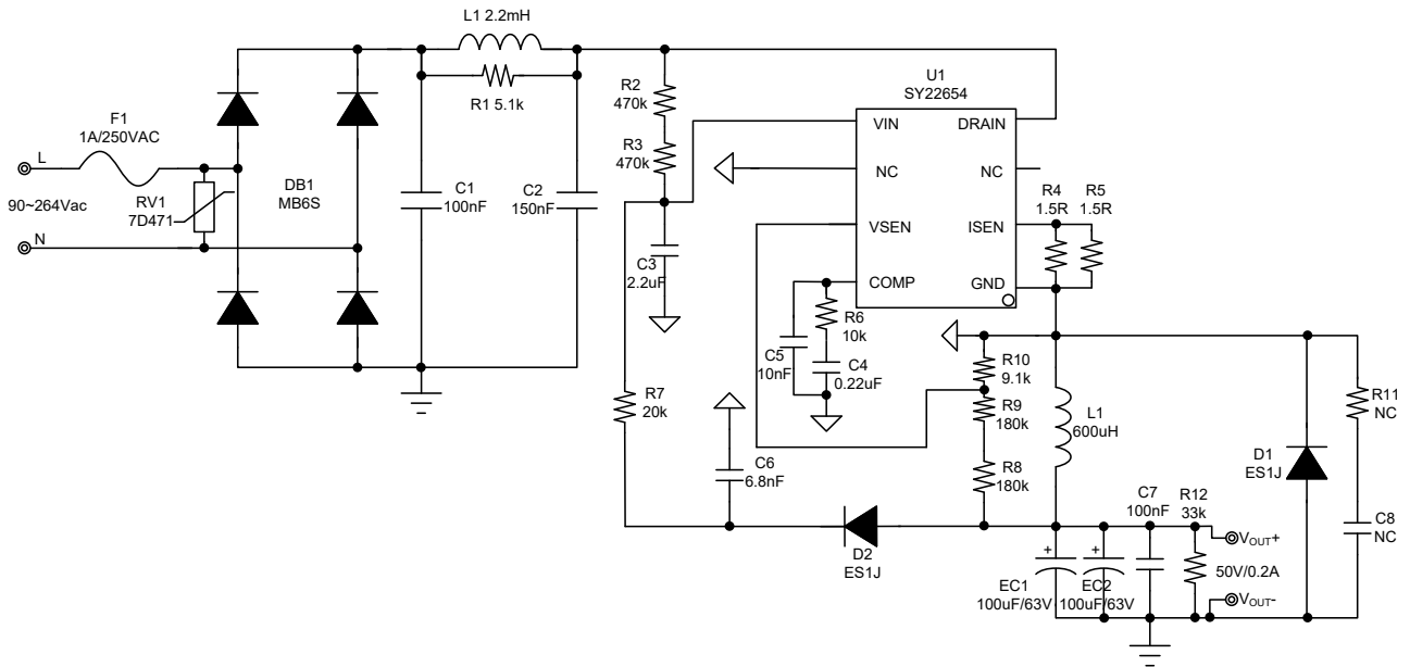
(b) Floating-switch Buck circuit @ 90~264Vac Input, 50V/0.2A Output
