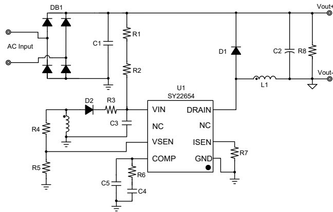
Fig. 1 Schematic Diagram
