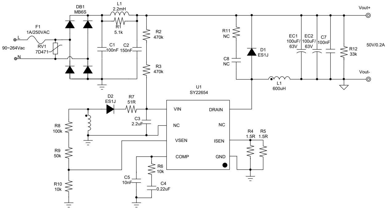
(a) Ground-switch Buck circuit @ 90~264Vac Input, 50V/0.2A Output
