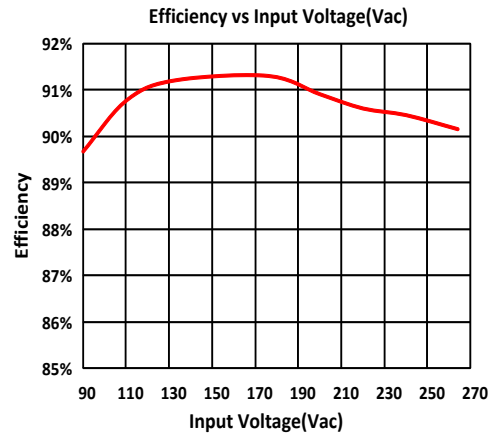
Fig. 2 Efficiency vs Input Voltage
