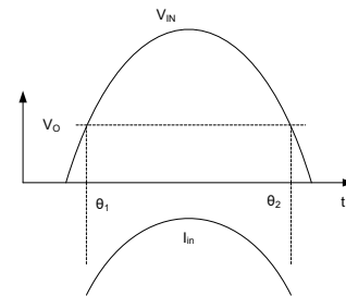
Fig.11 Input waveforms
