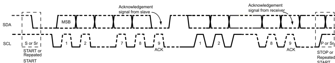
Figure 4. Data Transfer on the I²C Bus
