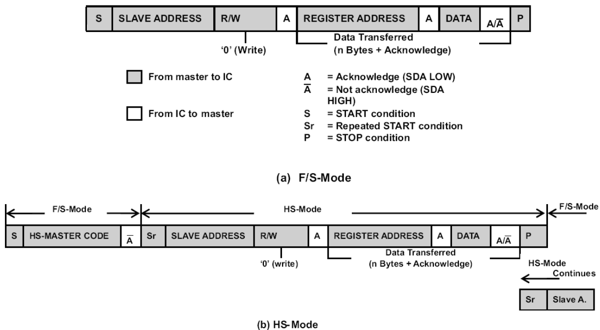
Figure 6. Bus Protocol
