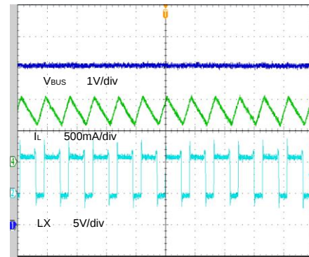
Boost Mode Full Load State
