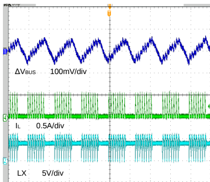
Boost Mode Light Load State
