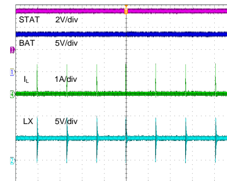
Time (20μs/div)
