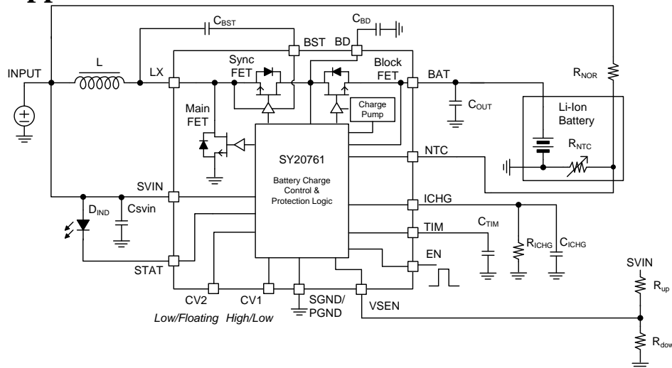
Figure1. Schematic Diagram
