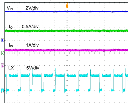
Time (1μs/div)
