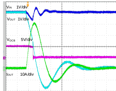
SY20807Z Short Circuit Response
