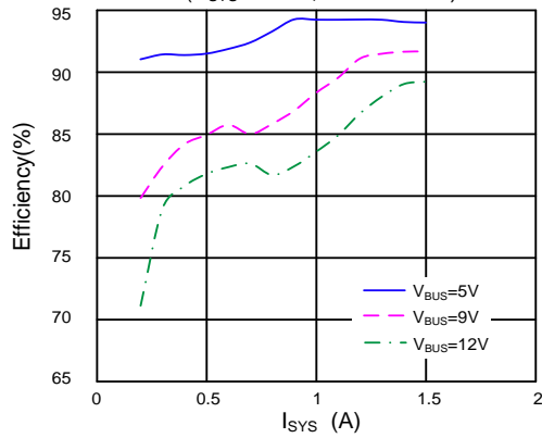
Efficiency vs. I_{\text{SYS}} (Charge Disable) ( V_{\text{SYS}}=3.65\text{V} , \text{DCR}=10\text{m}\Omega )
