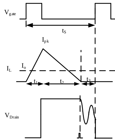
Fig.13 switching waveforms
