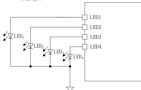
Figure 5. LED Configuration for Status Indicators
