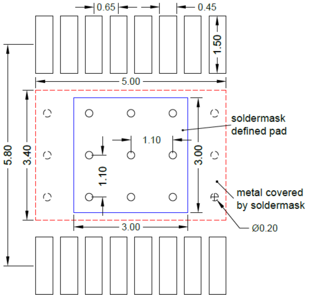
Recommended PCB layout (Reference only)
