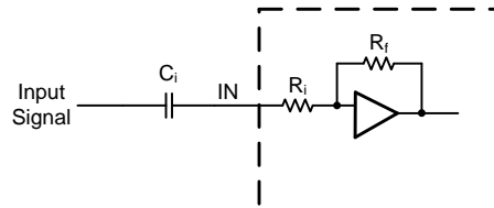
Figure 11. Input Impedance
