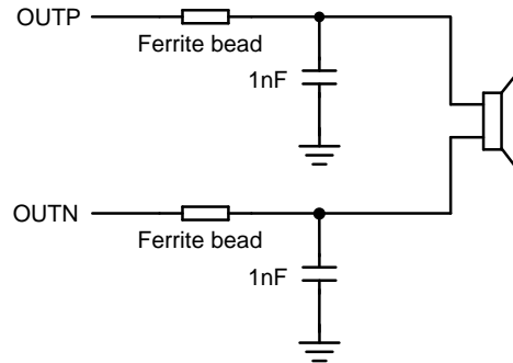
Figure 15. Typical Ferrite Bead EMI Filter
