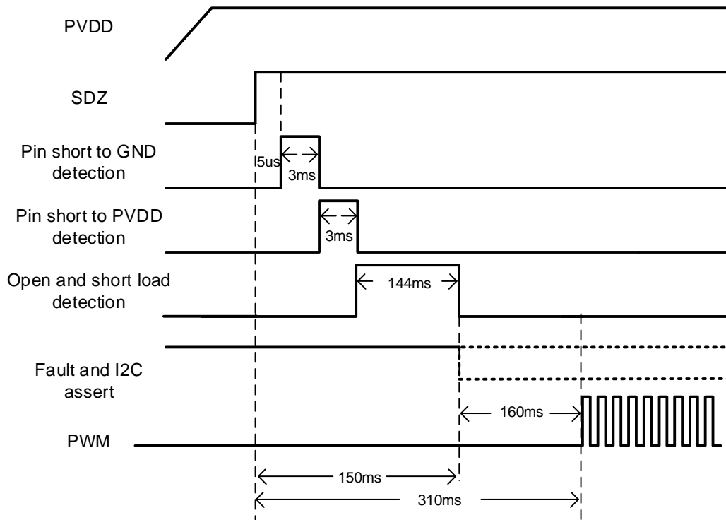
Figure 6. Load Diagnostics Timing
