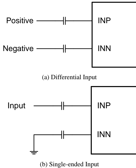
Figure 13. Input Signal Connection
