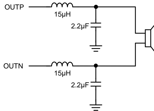
Figure 14. Typical LC output filter, Cutoff Frequency is 27 kHz, Speaker Impedance = 4Ω
