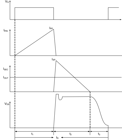
Fig.16 switching waveforms
