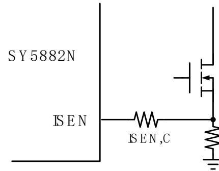
Fig.11 Feed-forward resistor
