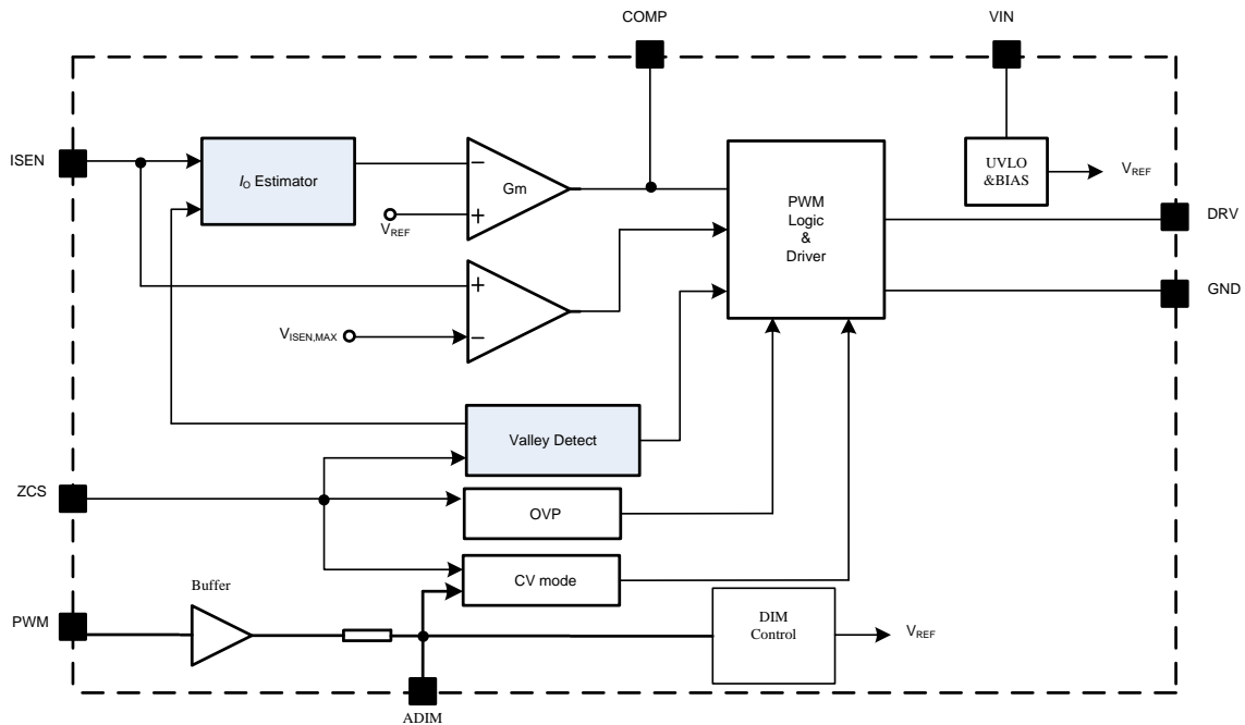
Figure.3 Block Diagram
