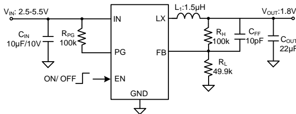
Figure1. Schematic Diagram
