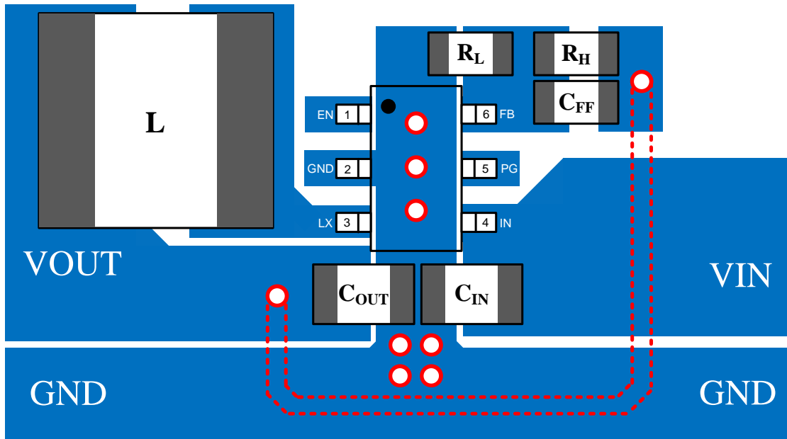
Figure4. PCB Layout Suggestion
