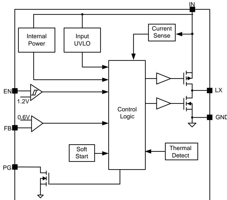
Figure3. Block Diagram
