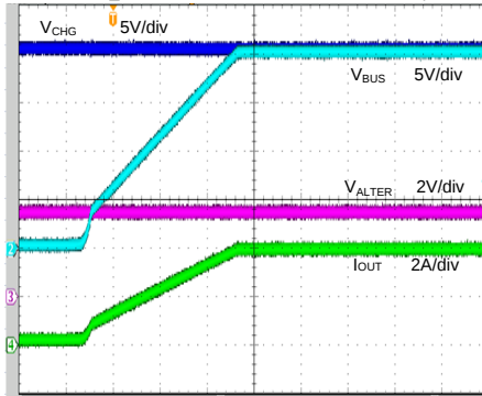
CHG_Source ON ( V_{CHG}=20V , V_{VSV}=5V , C_{CHG}=C_{BUS}=10\mu F , CHG\_ILIM=11 , OVP\_SET=111 , CHG Source mode, 5 \Omega Load)
