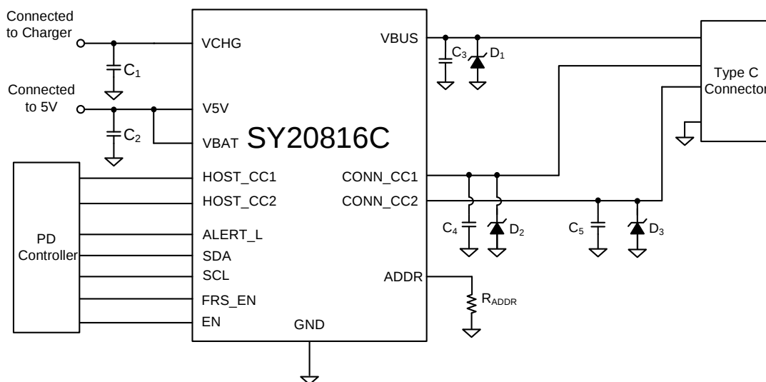
Figure 1. Schematic Diagram
