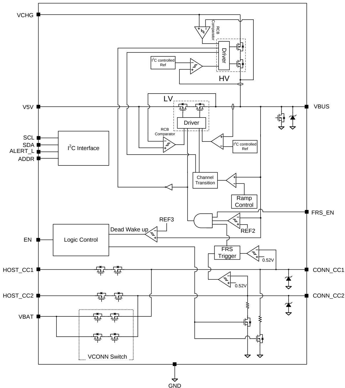
Figure 2. Block Diagram
