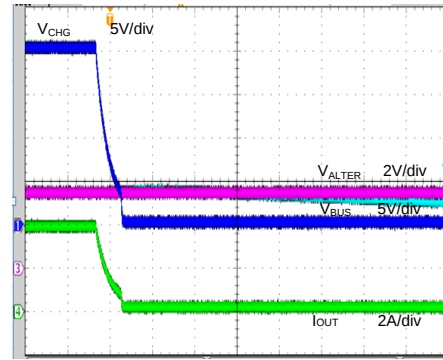
VBUS OFF ( V_{BUS}=20V , V_{VSV}=5V , C_{CHG}=C_{BUS}=10\mu F , CHG\_ILIM=11 , OVP\_SET=111 , CHG Sink mode, 5 \Omega Load)
