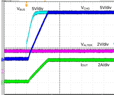
VBUS ON ( V_{BUS}=20V , V_{VSV}=5V , C_{CHG}=C_{BUS}=10\mu F , CHG\_ILIM=11 , OVP\_SET=111 , CHG Sink mode, 5 \Omega Load)
