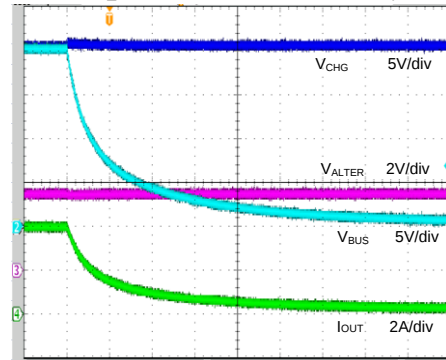
CHG_Source OFF ( V_{CHG}=20V , V_{VSV}=5V , C_{CHG}=C_{BUS}=10\mu F , CHG\_ILIM=11 , OVP\_SET=111 , CHG Source mode, 5 \Omega Load)
