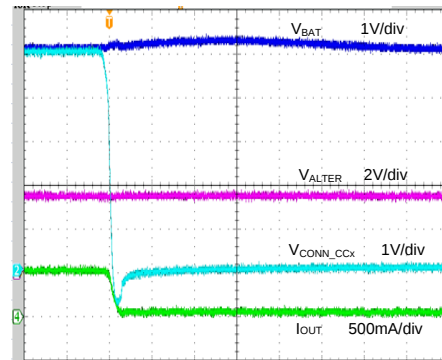
VCONN Switch OFF ( V_{BAT}=5V , C_{BAT}=1\mu F , VCONN=0 , 10 \Omega Load)
