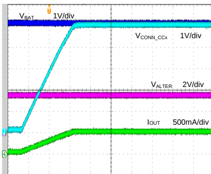
VCONN Switch ON ( V_{BAT}=5V , C_{BAT}=1\mu F , VCONN=1 , 10 \Omega Load)
