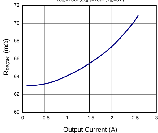
R_{DS(ON)} vs. Output Current ( C_{IN}=10\mu F, C_{OUT}=10\mu F, V_{IN}=5V )
