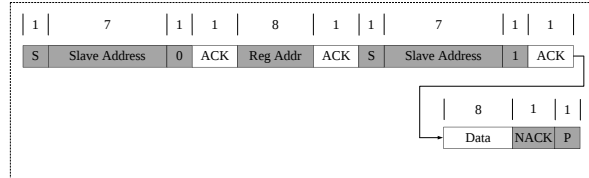
Figure 17. Single Read
