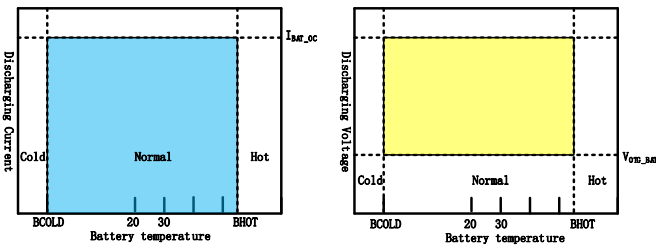
Figure 11. Temperature Window in Boost Mode
