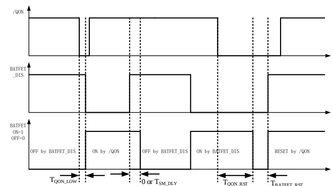
Figure 8. /QON Timing
