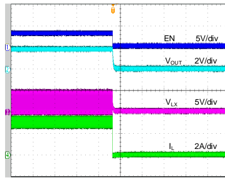
Time (800μs/div)
