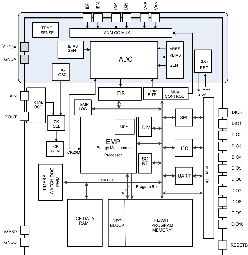
Figure 1. SY7T611+U2/I2 Functional Block Diagram
