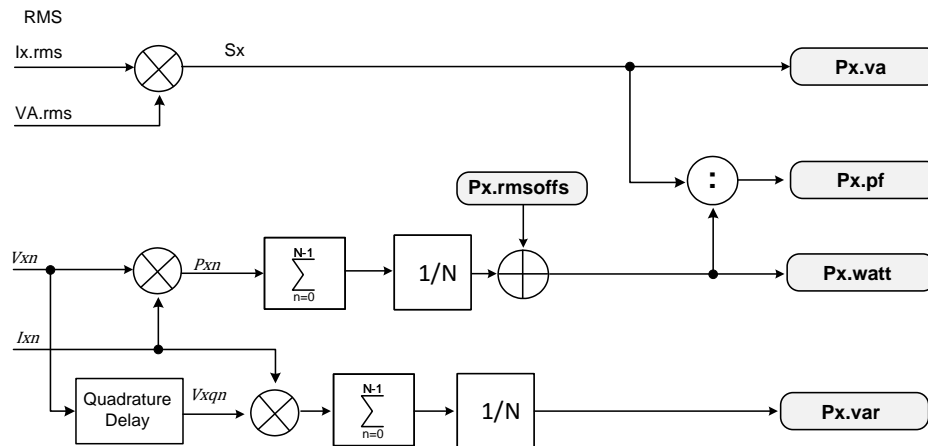
Figure 19: Power (Active, Reactive, and Apparent) and Power Factor Calculation
