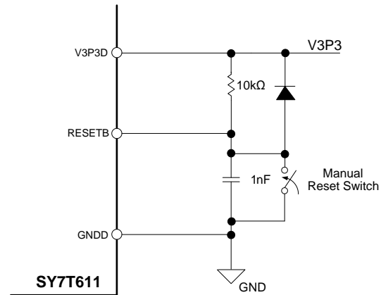
a) RESETB External Connection Example
