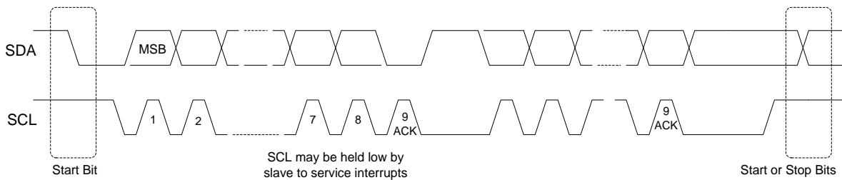
Figure 10: I 2 C Bus Conditions
