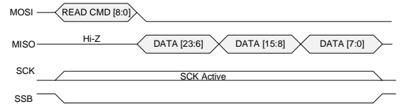
Figure 7. Single Word Read Access Timing
