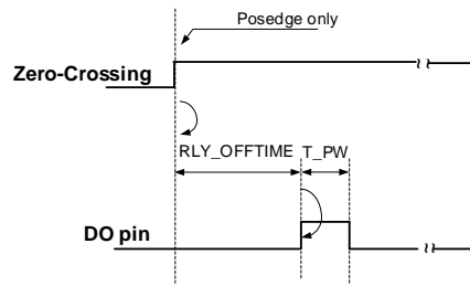
b. Relay De-activation (OFF Command)
