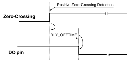
b. Relay De-activation (OFF Command)
