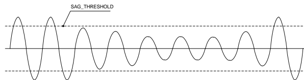
Figure 21. Voltage Sag
