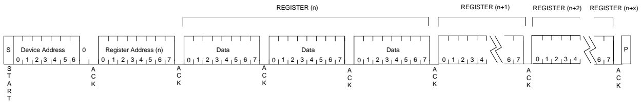
Figure 12: I 2 C Bus Multiple Sequential Register Write
