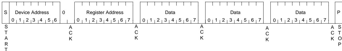
Figure 11: I 2 C Bus 3-byte Data Write
