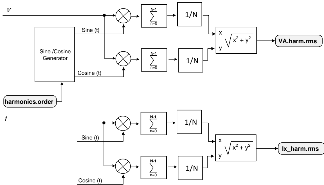
Figure 20: Voltage and Current Fundamental and Harmonic Calculations
