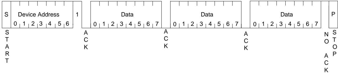
Figure 13: I 2 C Bus 3-byte Data Read
