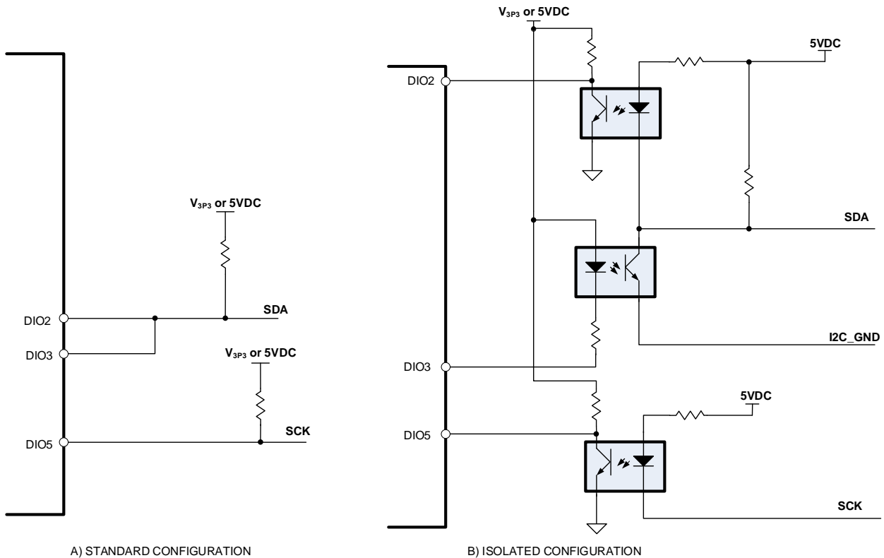
Figure 9: I 2 C Bus Connection in Standard (A) and Isolated (B) Configuration
