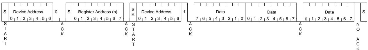
Figure 14: I 2 C Bus 3-byte Random Data Read
