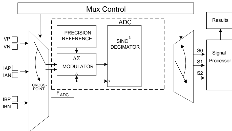
Figure 15. SY7T611 Analog Front-End
