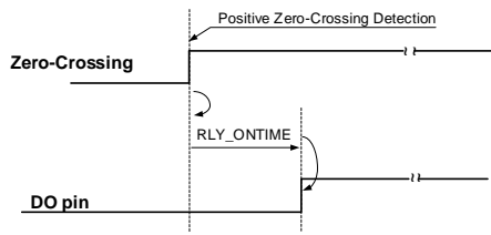
a. Relay Activation (ON Command)
