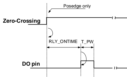
a. Relay Activation (ON Command)
