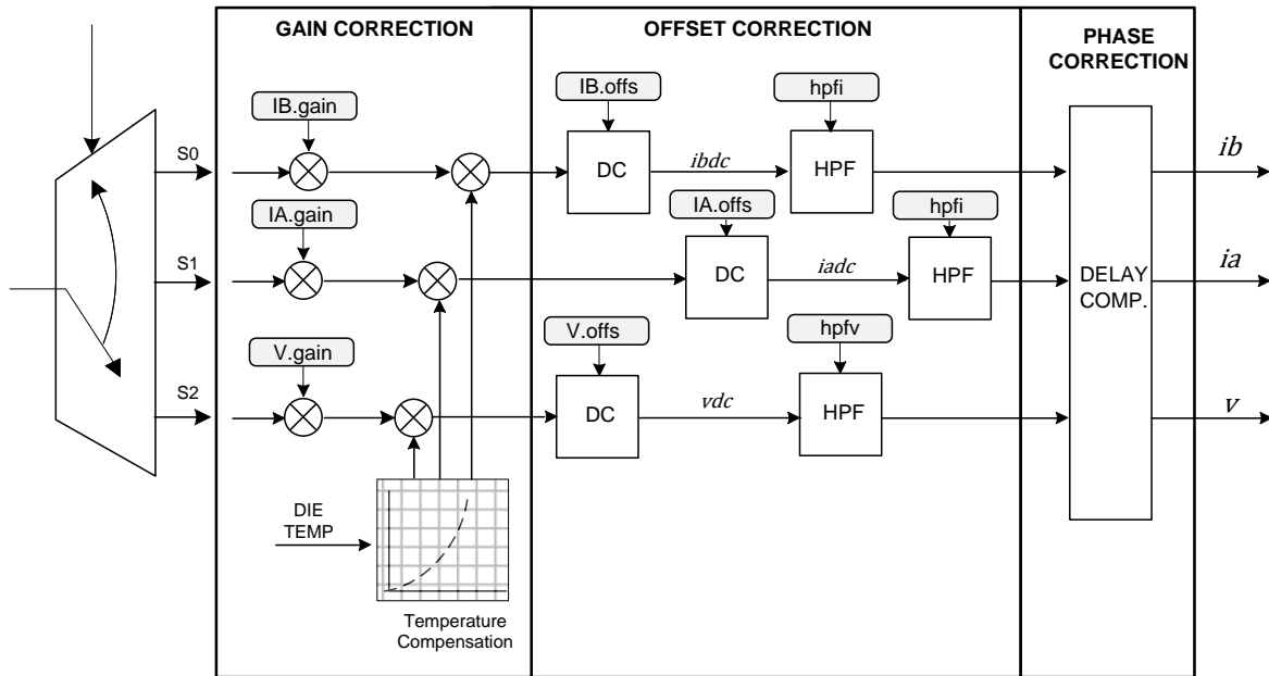
Figure 16: Analog Input Signal Conditioning
