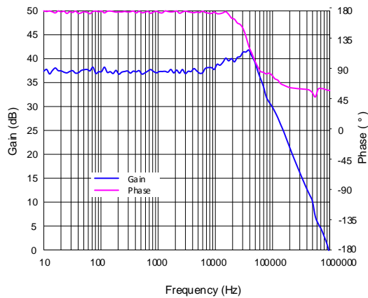
Bode Plot of VO Sink 1A ( V_{IN}=3.3V , V_{REFIN}=1.5V , sink 1A load)
