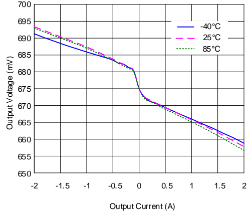
VO Load Regulation (0.675 V) ( V_N=3.3V , V_{REFIN}=1.35V )
