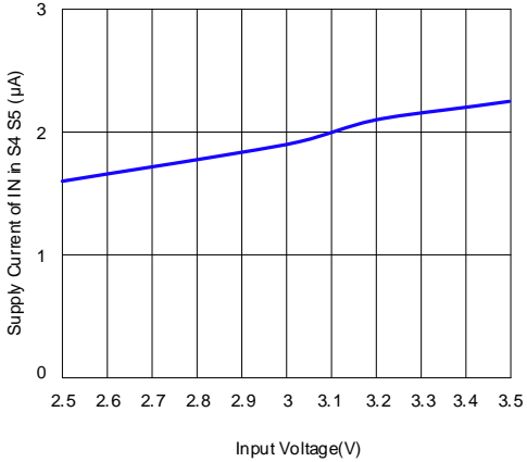
Supply Current of VIN in S4 S5 vs. Input Voltage ( V_{S3}=V_{S5}=0V , V_{REFIN}=1.8V )
