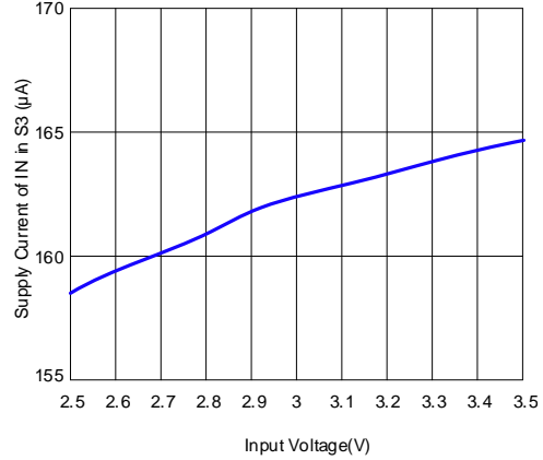
Supply Current of VIN in S3 vs. Input Voltage ( V_{S3}=0V , V_{S5}=3V , V_{REFIN}=1.8V )
