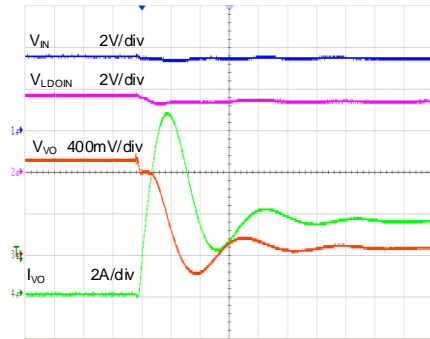
Short Circuit Response ( V_{IN}=V_{LDON}=3.5V , V_{REFIN}=1.8V )
