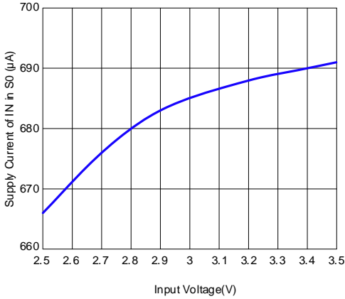
Supply Current of VIN in S0 vs. Input Voltage ( V_{S3}=V_{S5}=3V , V_{REFIN}=1.8V )
