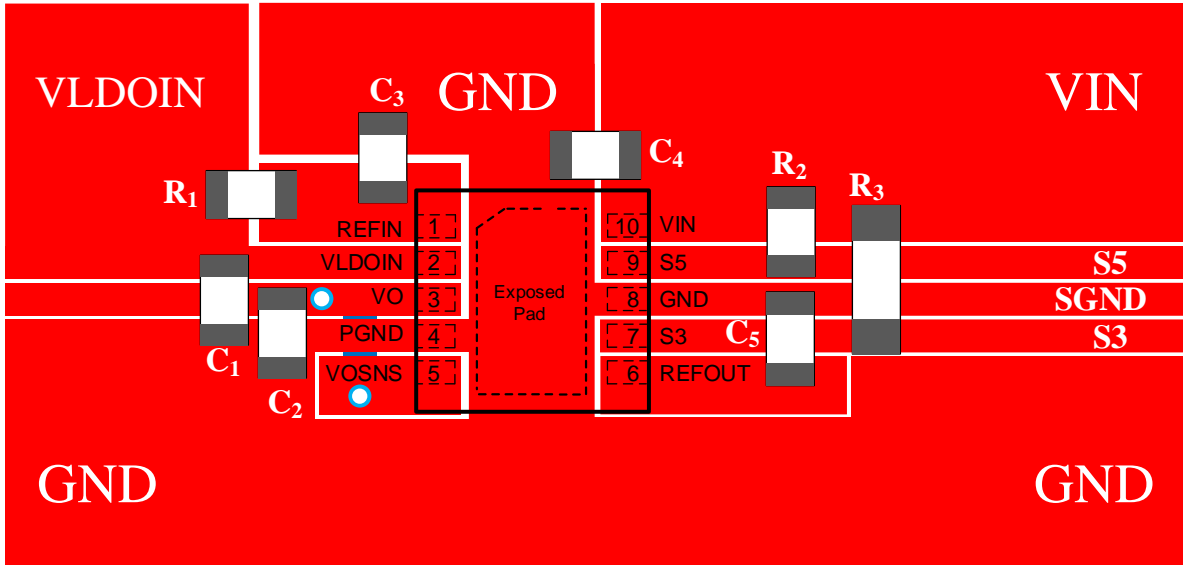
Figure 4. SY6355B PCB Layout Suggestion
