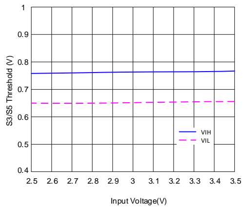
S3/S5 Threshold vs. Input Voltage ( V_{REFIN}=1.8V )
