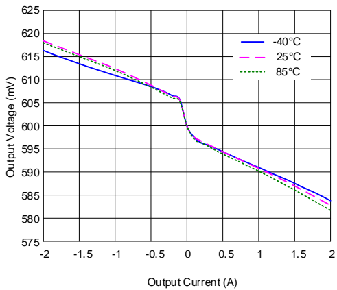
VO Load Regulation (0.6 V) ( V_N=3.3V , V_{REFIN}=1.2V )
