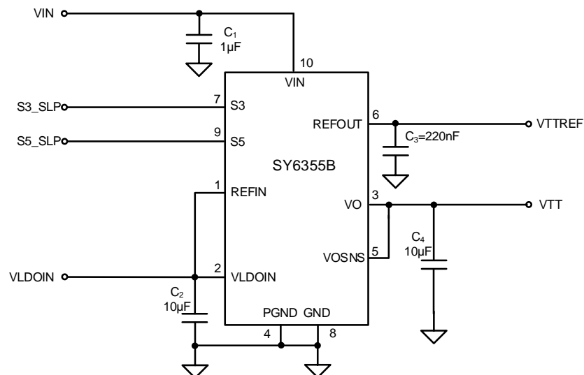
Figure 1. Schematic Diagram
