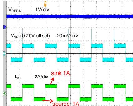
VO Load Transient Response (0.75 V) ( V_{IN}=3.3V , V_{REFIN}=1.5V )
