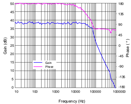
Bode Plot of VO Source 1A ( V_{IN}=3.3V , V_{REFIN}=1.5V , source 1A load)
