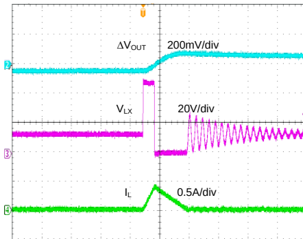
Output Ripple ( V_{IN}=48\text{V}, V_{OUT}=12\text{V}, I_O=0\text{A} )
