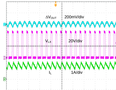
Output Ripple ( V_{IN}=48\text{V}, V_{OUT}=12\text{V}, I_O=1.2\text{A} )
