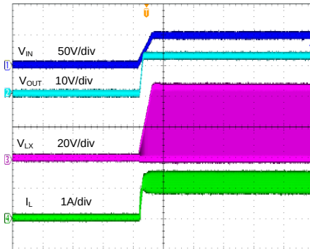
Startup from V_{IN} ( V_{IN}=48V , V_{OUT}=12V , I_O=1.2A )
