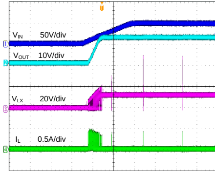
Startup from V_{IN} ( V_{IN}=48V , V_{OUT}=12V , I_O=0A )
