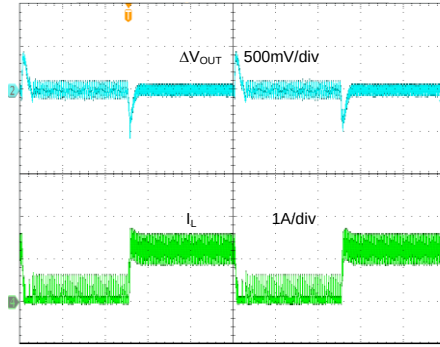
Load Transient ( V_{IN}=48\text{V}, V_{OUT}=12\text{V}, I_O=0.12 \sim 1.2\text{A} )
