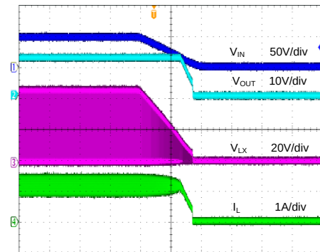
Shutdown from V_{IN} ( V_{IN}=48V , V_{OUT}=12V , I_O=1.2A )
