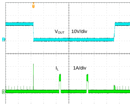
Hard Short Protection ( V_{IN}=48V , V_{OUT}=12V , I_O=0A \sim Short)
