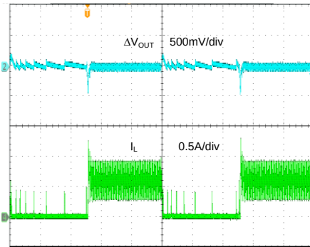
Load Transient ( V_{IN}=48\text{V}, V_{OUT}=12\text{V}, I_O=0 \sim 0.6\text{A} )
