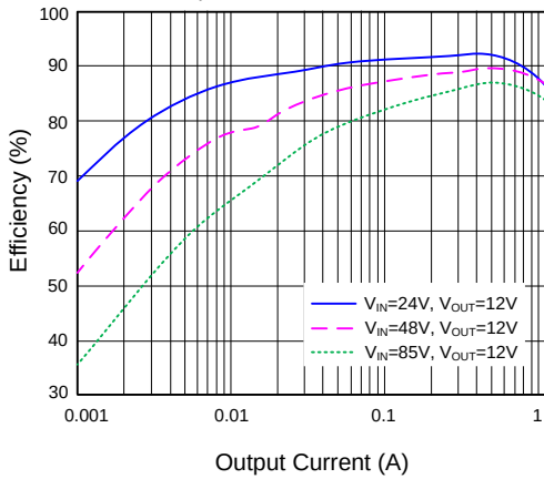
Efficiency vs. Output Current ( L=68\mu\text{H}/\text{CDRH8D43-680NC} )
