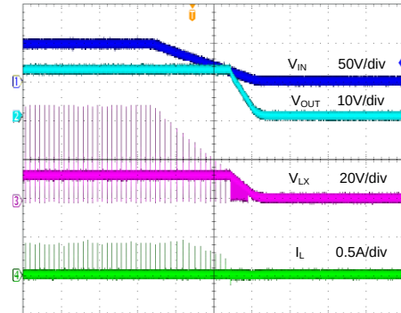
Shutdown from V_{IN} ( V_{IN}=48V , V_{OUT}=12V , I_O=0A )
