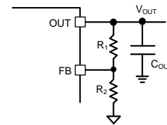
Fig. 5. V_{OUT} Programming
