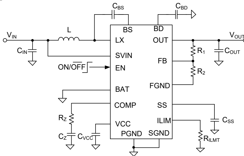
Figure 1. Schematic Diagram
