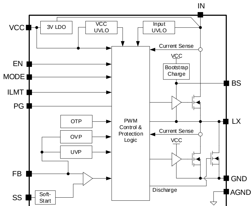
Figure 3. Block Diagram
