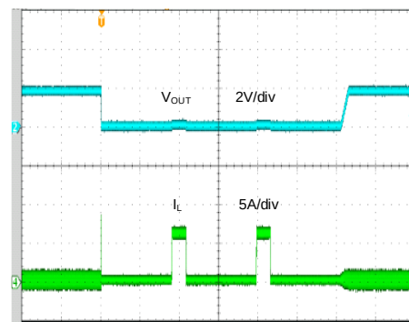
Short Circuit Protection ( V_{IN}=5V, V_{OUT}=1.8V, I_{OUT}=0A \sim Short FCCM)
