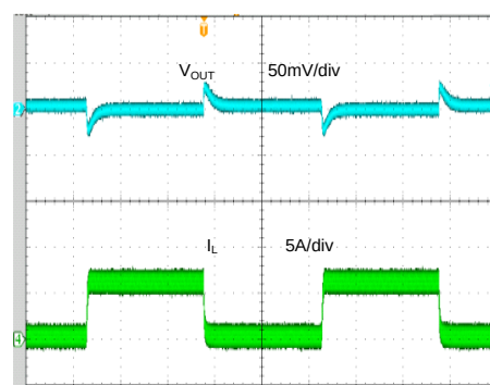
Load Transient ( V_{IN}=5V, V_{OUT}=1.8V, I_{OUT}=0A \sim 6A , FCCM)
