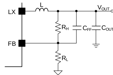
Figure 8. Feed-Forward Capacitor
