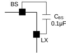
Figure 5. Bootstrap Capacitor Connection
