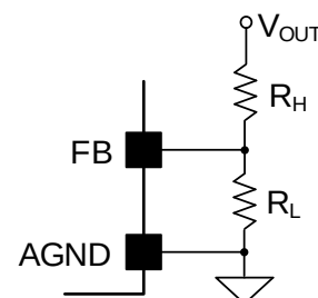
Figure 7. Feedback Resistor
