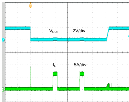
Short Circuit Protection ( V_{IN}=5V, V_{OUT}=1.8V, I_{OUT}=0A \sim Short PFM)
