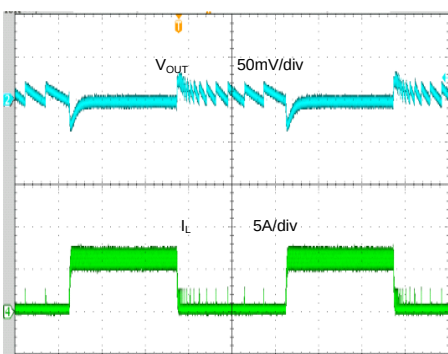
Load Transient ( V_{IN}=5V, V_{OUT}=1.8V, I_{OUT}=0A \sim 6A , PFM)
