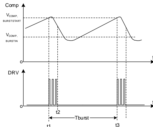
Figure 4. Quiet Burst
