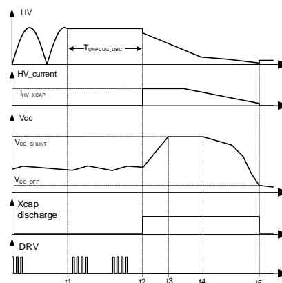
Figure 14. X Capacitor Discharge Waveforms
