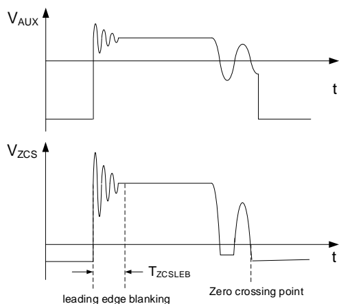
Figure 3. Valley Detection
