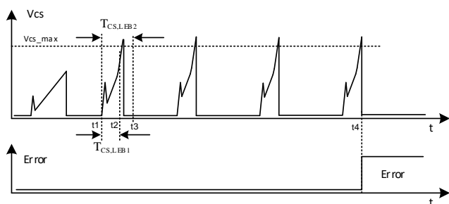
Figure 12. V_{CS\_MAX} Process
