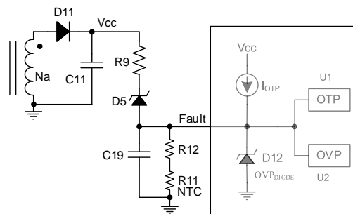
Figure 17. Fault OTP and OVP
