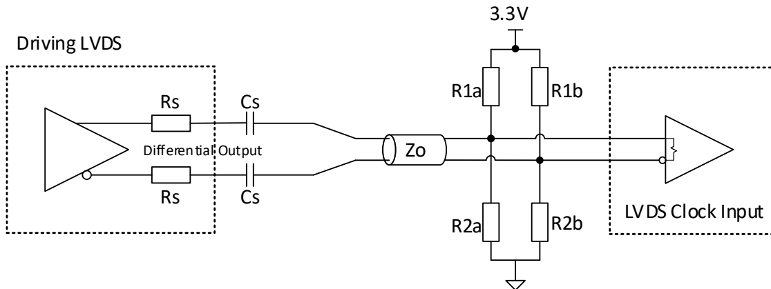
Figure 8. Differential Output Driving LVDS
