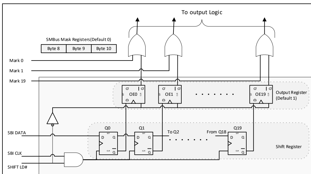
Figure 3. Side-Band Interface
