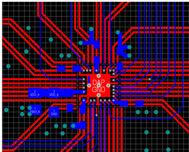
Figure 11. Layout Recommendation
