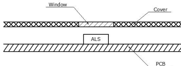
Figure 5. Ambient Light Sensor Mounted Inside an Apparatus
