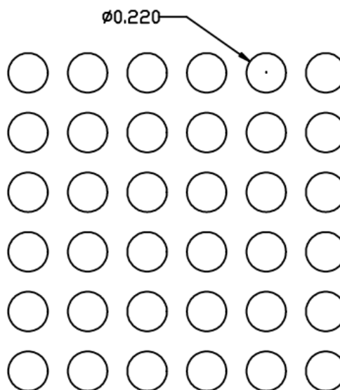
Recommended PCB layout (Reference only)
