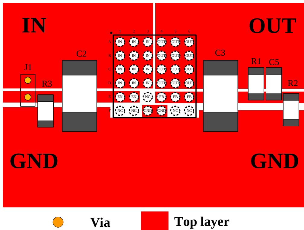
Figure4. PCB Layout Suggestion
