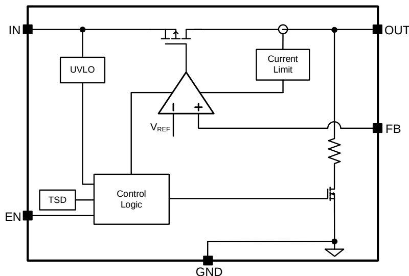
Figure2. Block Diagram
