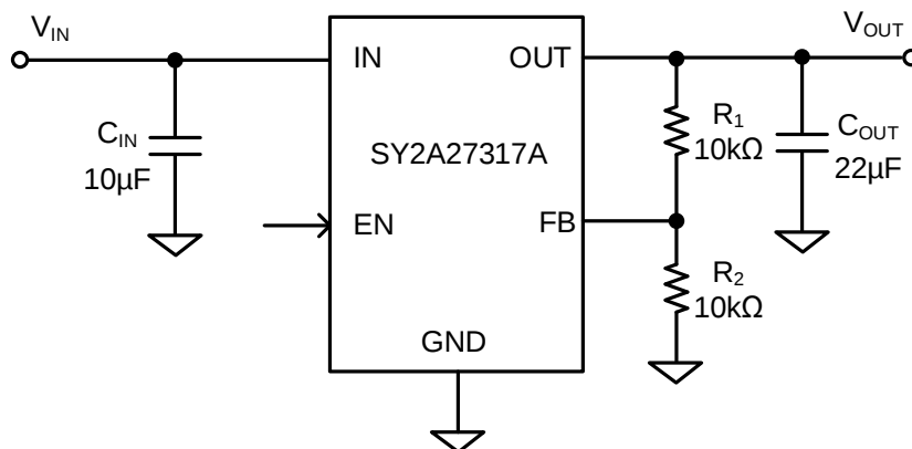
Figure1. Schematic Diagram
