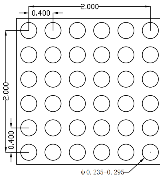
Bottom View
