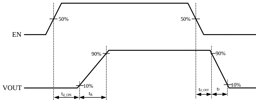
Figure 3. Power ON/OFF Timing Definition
