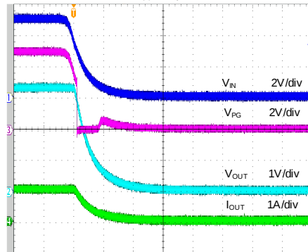
Shutdown from V_{IN} ( V_{IN}=5V , V_{OUT}=3.3V , SS\_CTRL=GND , C_N=10\mu F , C_{OUT}=22\mu F , I_{OUT}=1A )
