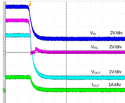
Shutdown from V_{IN} ( V_{IN}=5V , V_{OUT}=3.3V , SS\_CTRL=V_{IN} , C_N=10\mu F , C_{OUT}=22\mu F , I_{OUT}=1A )
