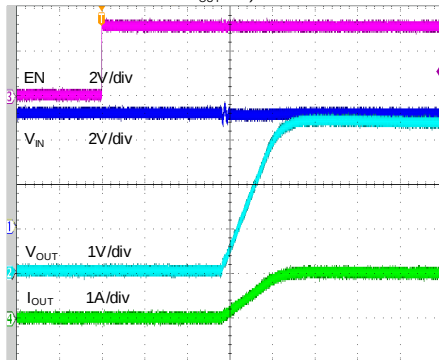
Startup from EN ( V_{IN}=5V , V_{OUT}=3.3V , SS\_CTRL=V_{IN} , C_N=10\mu F , C_{OUT}=22\mu F , I_{OUT}=1A )
