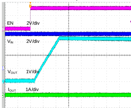
Startup from EN ( V_{IN}=5V , V_{OUT}=3.3V , SS\_CTRL=GND , C_N=10\mu F , C_{OUT}=22\mu F , Null Load)
