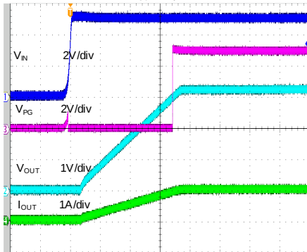
Startup from V_{IN} ( V_{IN}=5V , V_{OUT}=3.3V , SS\_CTRL=GND , C_N=10\mu F , C_{OUT}=22\mu F , I_{OUT}=1A )
