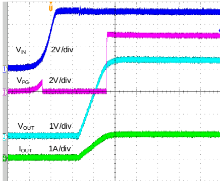
Startup from V_{IN} ( V_{IN}=5V , V_{OUT}=3.3V , SS\_CTRL=V_{IN} , C_N=10\mu F , C_{OUT}=22\mu F , I_{OUT}=1A )
