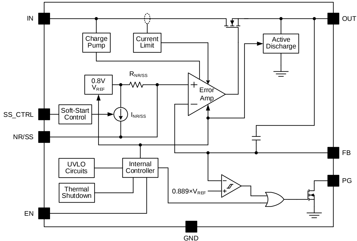
Figure2. Block Diagram
