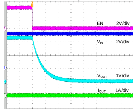
Shutdown from EN ( V_{IN}=5V , V_{OUT}=3.3V , SS\_CTRL=GND , C_N=10\mu F , C_{OUT}=22\mu F , Null Load)
