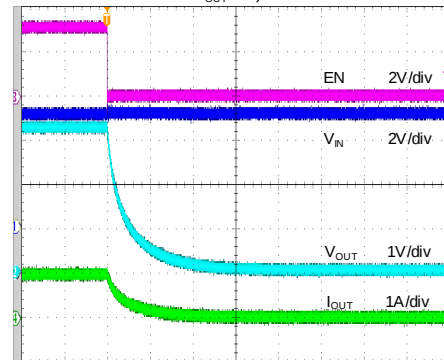
Shutdown from EN ( V_{IN}=5V , V_{OUT}=3.3V , SS\_CTRL=V_{IN} , C_N=10\mu F , C_{OUT}=22\mu F , I_{OUT}=1A )
