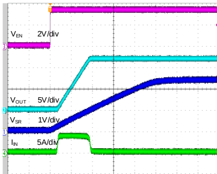
Turn ON with Enable ( V_{IN}=12V , V_{VCC}=3V , C_{SR}=100nF , C_{OUT}=100nF , 5mF Load)
