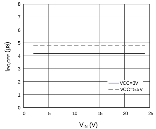
Power Good Turn-off Time vs. Input Voltage
