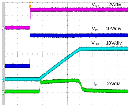
Hot Plug ( V_{IN} ) ( V_{IN}=24V , V_{VCC}=V_{EN}=6V , C_{SR}=C_{IN}=Open , C_{OUT}=100\mu F )
