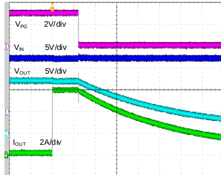
Over Current Protection ( V_{IN}=12V , V_{VCC}=3V , R_{OCP}=100k\Omega , C_{SR}=100nF , C_{OUT}=100nF , 5mF Load, Null Load \rightarrow 2\Omega )
