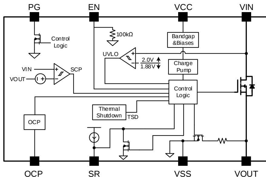
Figure 2 Block Diagram
