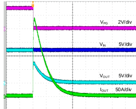
Hard Short ( V_{IN}=12V , V_{VCC}=3V , R_{OCP}=100k\Omega , C_{SR}=100nF , C_{OUT}=100nF , 5mF Load, Short OUT)
