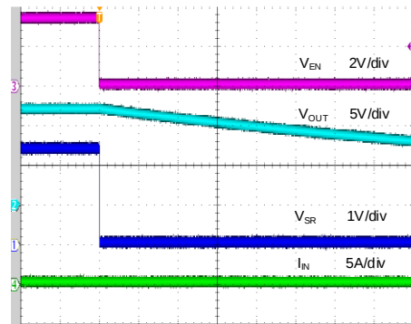
Turn OFF with Enable ( V_{IN}=12V , V_{VCC}=3V , C_{SR}=100nF , C_{OUT}=100nF , 5mF Load)
