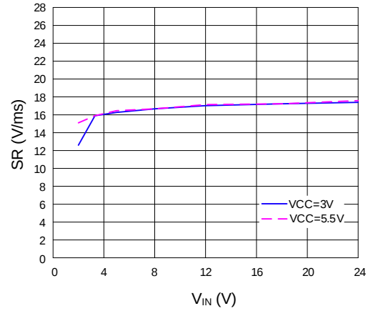
Output Slew Rate vs. Input Voltage
