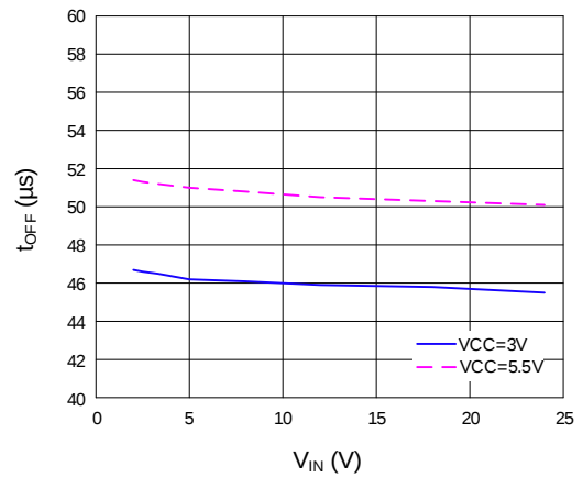
Output Turn-off Delay vs. Input Voltage
