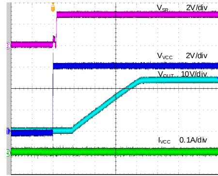
Hot Plug ( V_{VCC} ) ( V_{VCC}=V_{EN}=6V , V_{IN}=24V , C_{SR}=C_{VCC}=Open , C_{OUT}=100\mu F )
