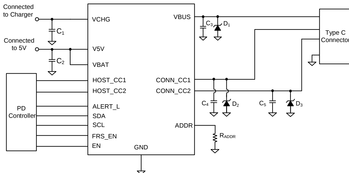
Figure 1. Schematic Diagram
