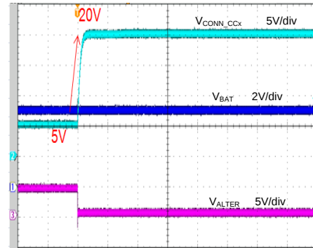
VBAT Over Voltage Protection Response ( V_{V5V}=V_{BAT}=5V , VCONN is enabled V_{CONN\_CC1Z}=5.0V \rightarrow 20.0V , C_{BAT}=1\mu F )
