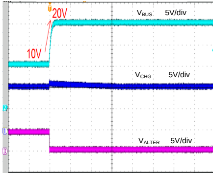
CHG Over Voltage Protection Response ( V_{V5V}=5V , V_{CHG}=10V , OVP\_SET=010 , V_{BUS}=10.0V \rightarrow 20.0V , CHG Source mode, C_{CHG}=C_{VBUS}=10\mu F )
