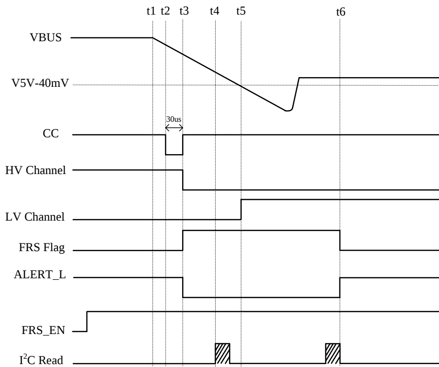
Figure 7. Timing Diagram on CC_FRS=0
