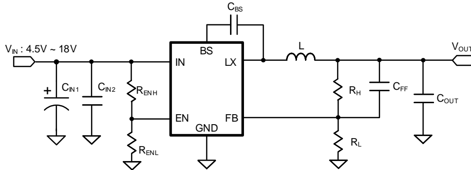
Figure8. Schematic Diagram
