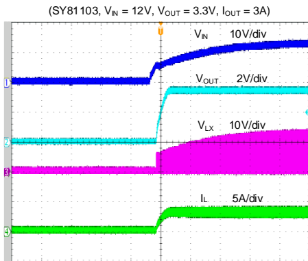
Startup from V_{IN}
