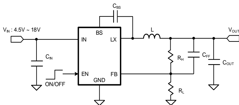
Figure 1. Schematic Diagram
