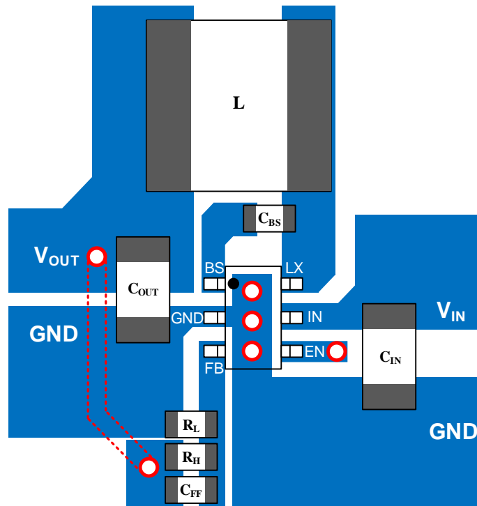
Figure 10. Suggested PCB Layout
