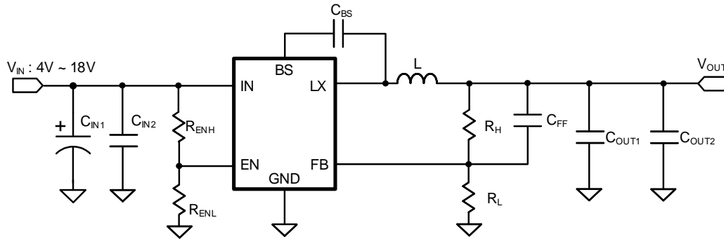
Figure8. Schematic Diagram
