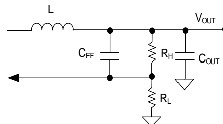
Figure7. Feedforward Network
