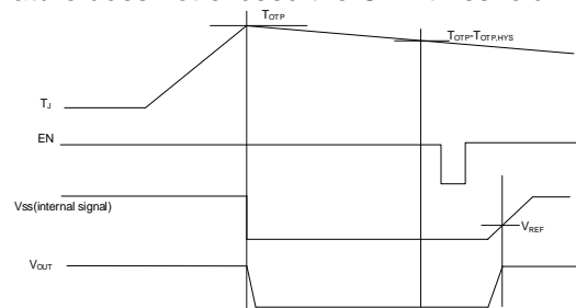
Figure12. Over Temperature Protection
