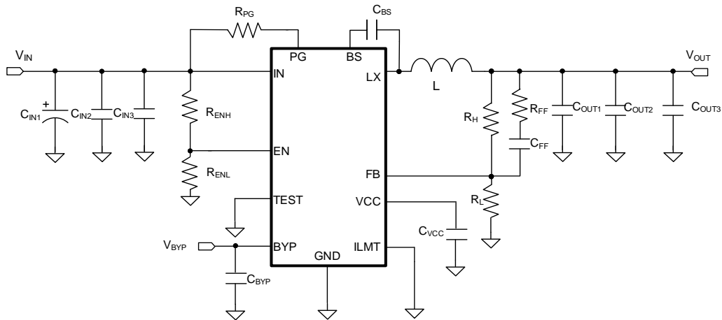
Figure15. Schematic Diagram
