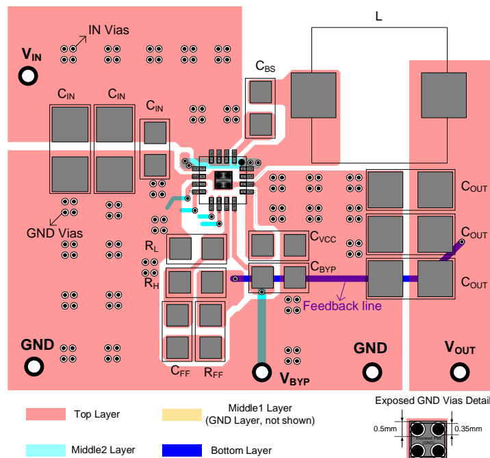
Figure16. PCB Layout Suggestion
