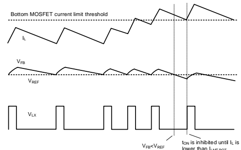
Figure 10. Bottom Current Limit Protection
