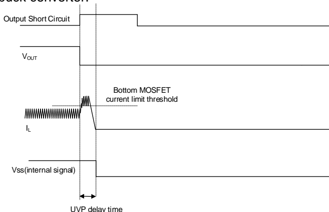
Figure11. Output Under Voltage Protection
