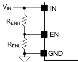
Figure 5. Enable Control
