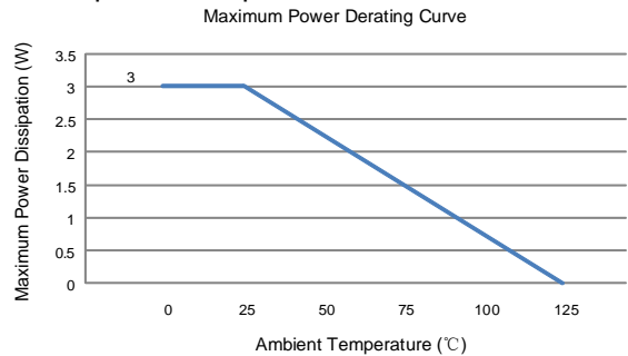
Figure14. Maximum Power Derating Curve
