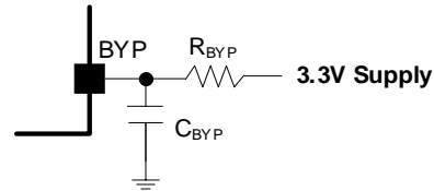
Figure 9. BYP Low Pass Filter Connection
