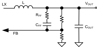
Figure13. Feedforward Network
