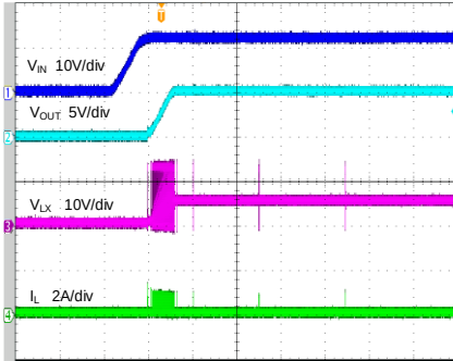
VIN ON (SA24483, V_{IN}=12V , V_{OUT}=5V , I_{OUT}=0A , f_{SW}=400kHz )
