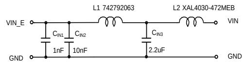
EMI Filter
