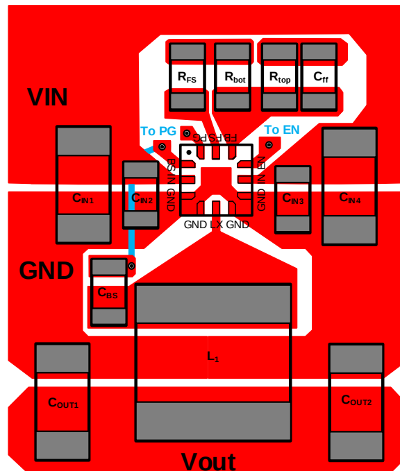
Figure 9. Suggested PCB Layout
