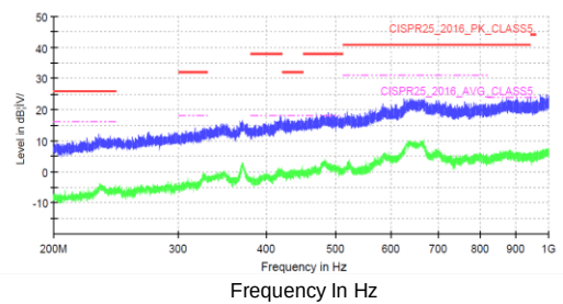
CISPR 25 Class 5 Radiated Emission (SA24483, I_{OUT}=3A , F_{SCAN}=200MHz-1GHz , Horizontal)
