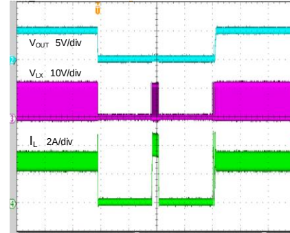
Short Circuit Protection (SA24483, V_{IN}=12V , V_{OUT}=5V , I_{OUT}=3A )
