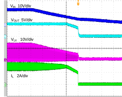
VIN OFF (SA24483, V_{IN}=12V , V_{OUT}=5V , I_{OUT}=3A , f_{SW}=400kHz )
