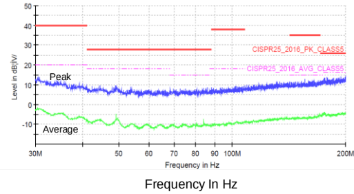
CISPR 25 Class 5 Radiated Emission (SA24483, I_{OUT}=3A , F_{SCAN}=30MHz-200MHz , Horizontal)
