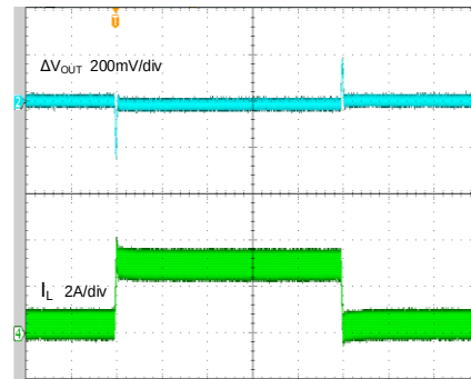
Load Transient (SA24483E, V_{IN}=12V , V_{OUT}=5V , I_{OUT}=0.3-3A )
