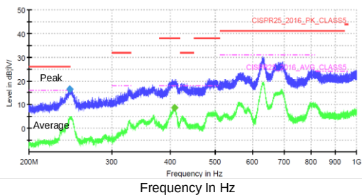
CISPR 25 Class 5 Radiated Emission (SA24483, I_{OUT}=3A , F_{SCAN}=200MHz-1GHz , Vertical)
