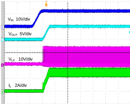
VIN ON (SA24483, V_{IN}=12V , V_{OUT}=5V , I_{OUT}=3A , f_{SW}=400kHz )
