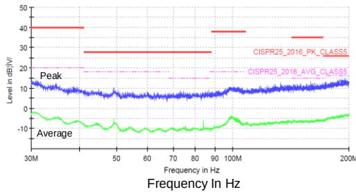
CISPR 25 Class 5 Radiated Emission (SA24483, I_{OUT}=3A , F_{SCAN}=30MHz-200MHz , Vertical)
