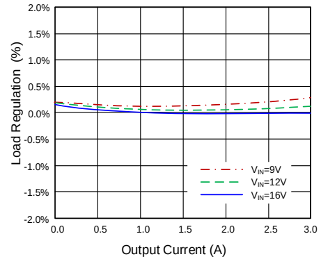
Load Regulation (SA24483E, V_{OUT}=5V , f_{SW}=400kHz , I_{OUT}=0-3A )
