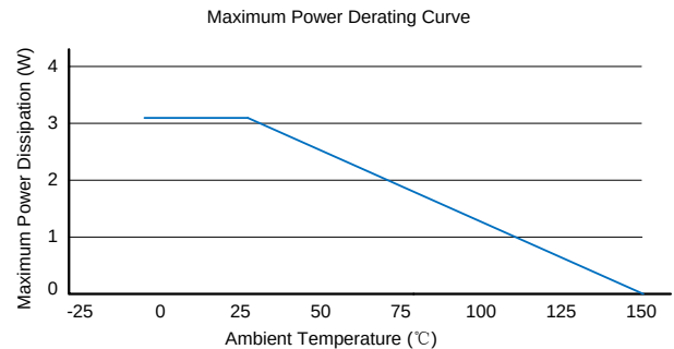
Figure 8. Derating Curve
