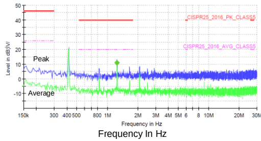
CISPR 25 Class 5 Radiated Emission (SA24483, I_{OUT}=3A , F_{SCAN}=150kHz-30MHz )
