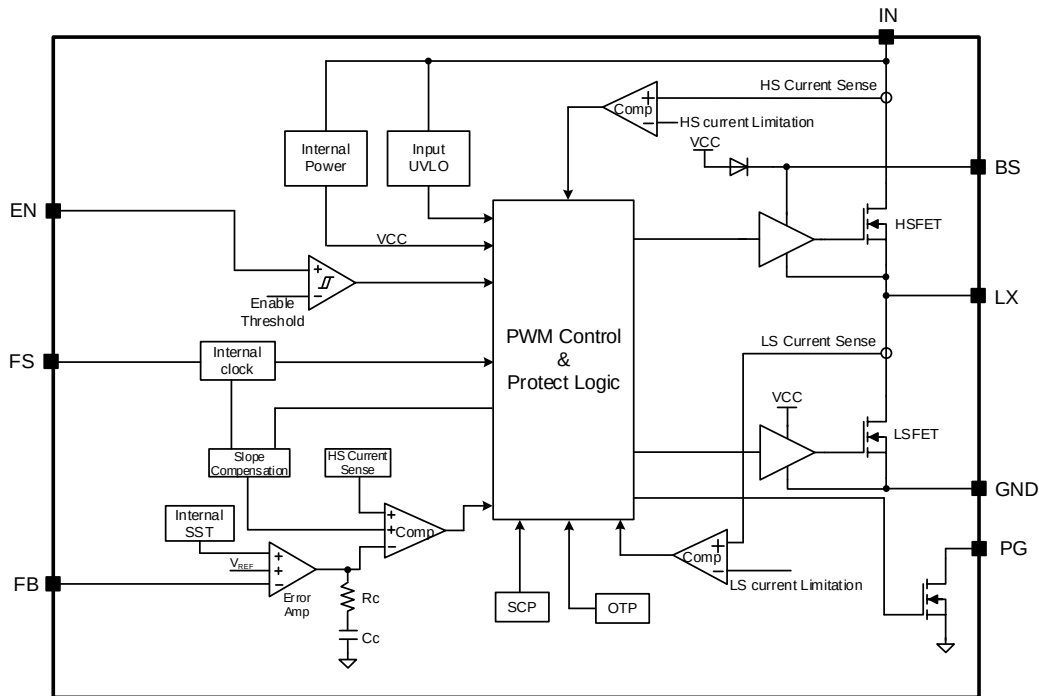
Figure 3. Block Diagram
