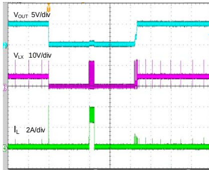
Short Circuit Protection (SA24483, V_{IN}=12V , V_{OUT}=5V , I_{OUT}=0A )
