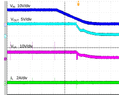
VIN OFF (SA24483, V_{IN}=12V , V_{OUT}=5V , I_{OUT}=0A , f_{SW}=400kHz )
