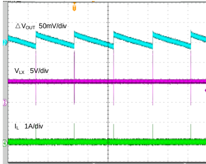
Output Ripple (SA24483, V_{IN}=12V , V_{OUT}=5V , I_{OUT}=0A )
