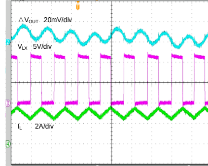
Output Ripple (SA24483, V_{IN}=12V , V_{OUT}=5V , I_{OUT}=3A )
