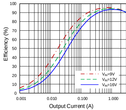
Efficiency vs. Output Current (SA24483E, V_{OUT}=5V , f_{SW}=400kHz , L=6.8\mu H /CMMB104T-6R8MS)
