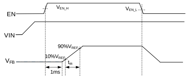
Figure 6. EN ON/OFF Sequence
